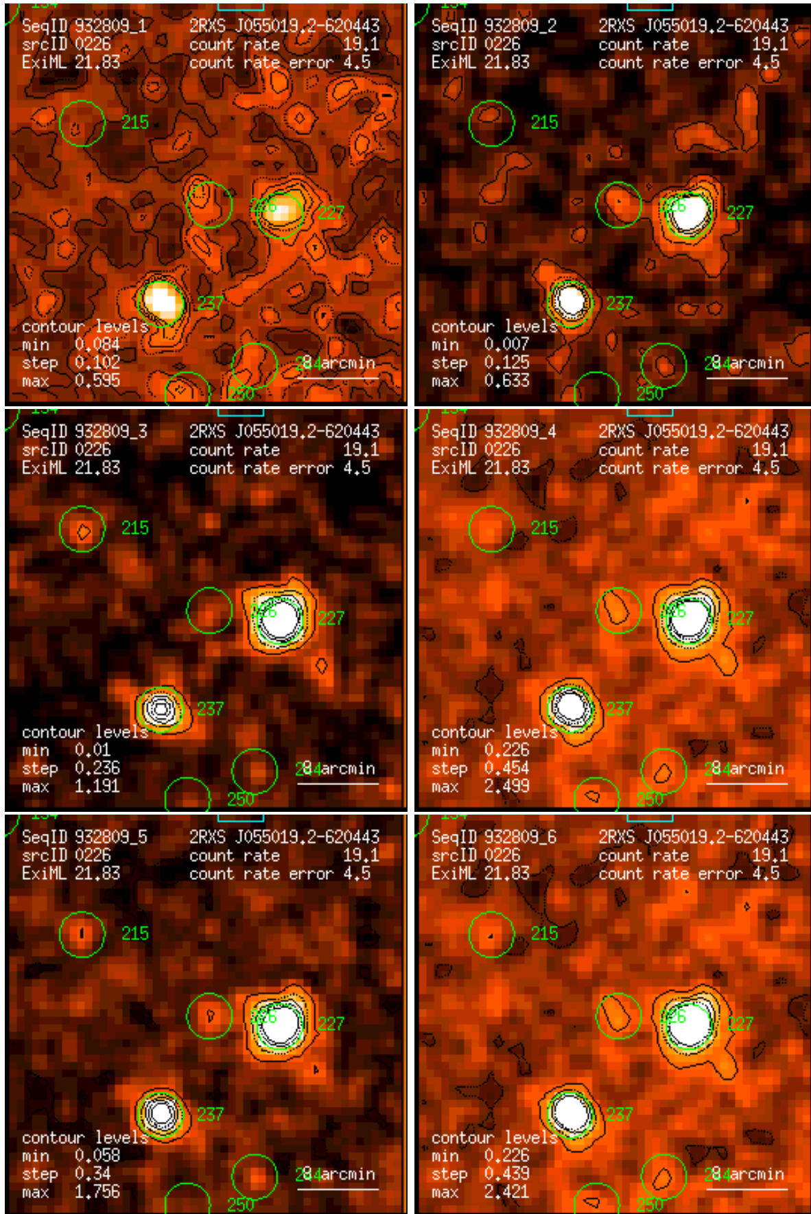
Figure 226: RASS 932809: detection 0226: band rate images, Gaussian filter: (1) PSPC channels 11 – 41, (2) 52 – 90, (3) 91 – 201, (4) 11 – 235, (5) 52 – 201, (6) 11 – 201. Broad band rates in counts/ks. Band rate contour levels in counts/ks/arcmin 2 .
