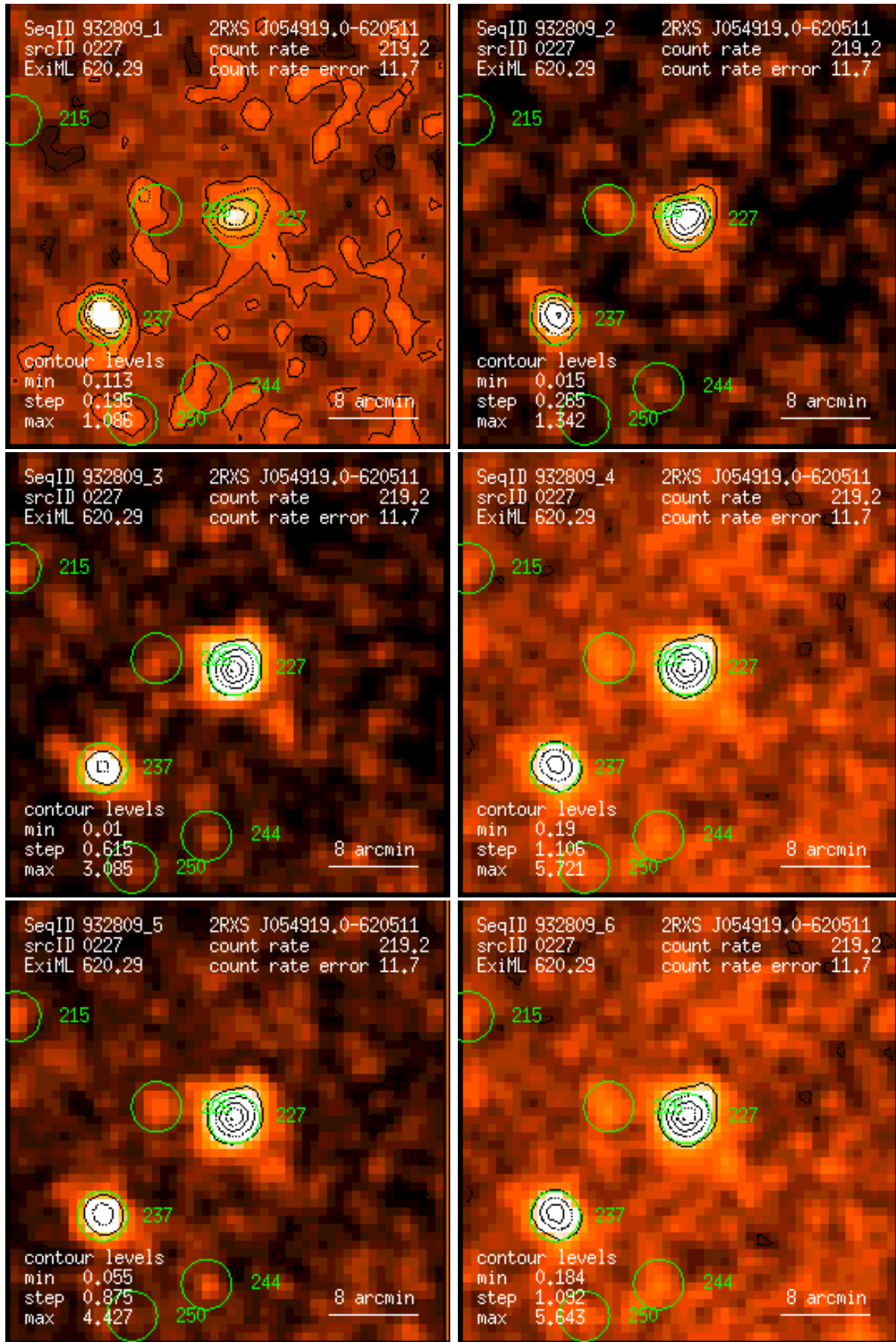
Figure 227: RASS 932809: detection 0227: band rate images, Gaussian filter: (1) PSPC channels 11 – 41, (2) 52 – 90, (3) 91 – 201, (4) 11 – 235, (5) 52 – 201, (6) 11 – 201. Broad band rates in counts/ks. Band rate contour levels in counts/ks/arcmin 2 .
