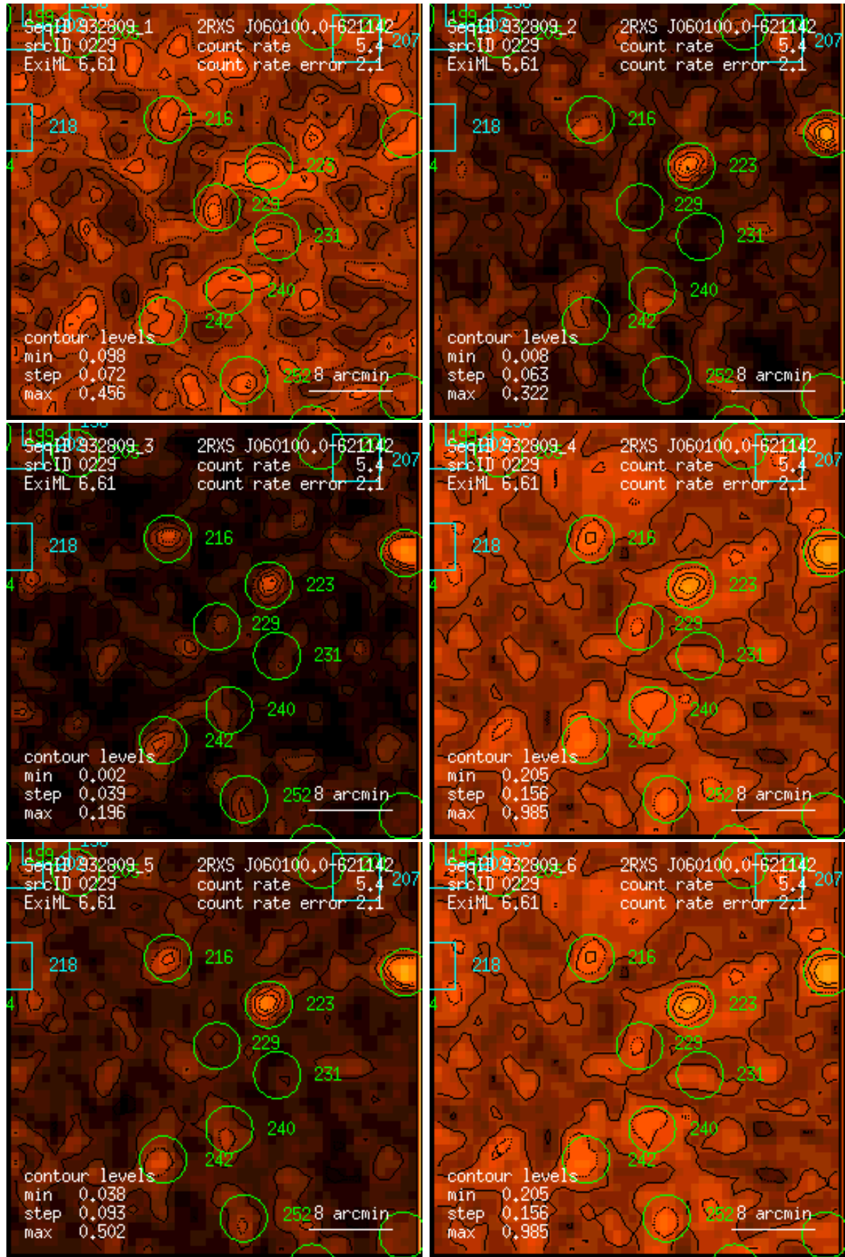
Figure 229: RASS 932809: detection 0229: band rate images, Gaussian filter: (1) PSPC channels 11 – 41, (2) 52 – 90, (3) 91 – 201, (4) 11 – 235, (5) 52 – 201, (6) 11 – 201. Broad band rates in counts/ks. Band rate contour levels in counts/ks/arcmin 2 .
