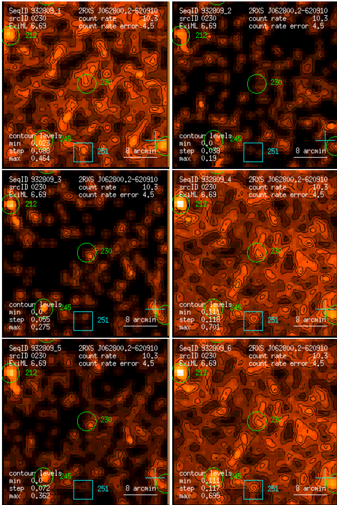
Figure 230: RASS 932809: detection 0230: band rate images, Gaussian filter: (1) PSPC channels 11 – 41, (2) 52 – 90, (3) 91 – 201, (4) 11 – 235, (5) 52 – 201, (6) 11 – 201. Broad band rates in counts/ks. Band rate contour levels in counts/ks/arcmin 2 .
