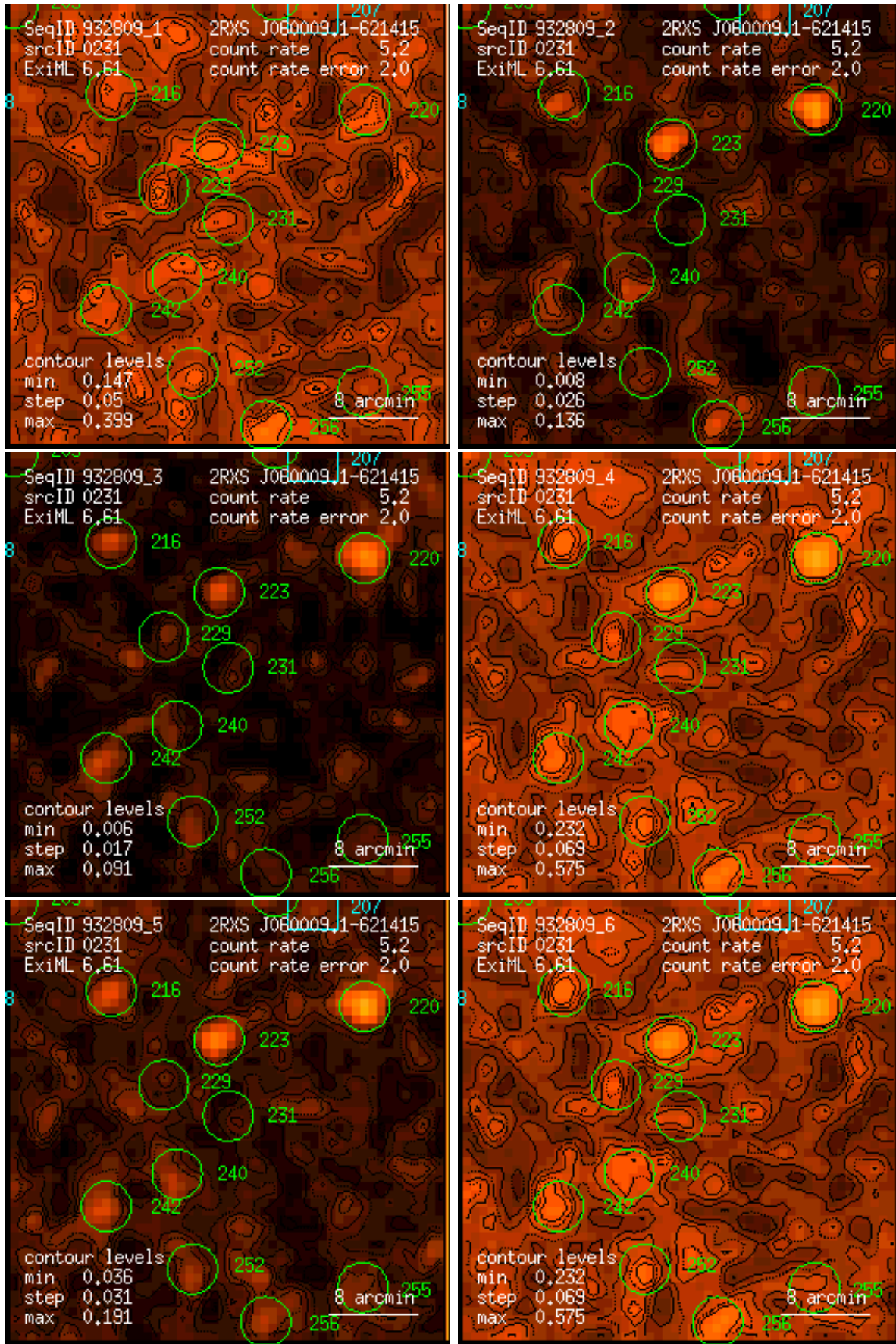
Figure 231: RASS 932809: detection 0231: band rate images, Gaussian filter: (1) PSPC channels 11 – 41, (2) 52 – 90, (3) 91 – 201, (4) 11 – 235, (5) 52 – 201, (6) 11 – 201. Broad band rates in counts/ks. Band rate contour levels in counts/ks/arcmin 2 .
