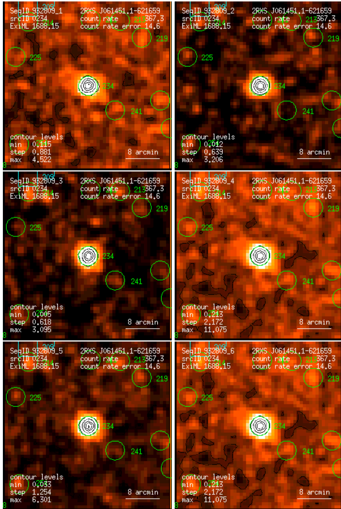
Figure 234: RASS 932809: detection 0234: band rate images, Gaussian filter: (1) PSPC channels 11 – 41, (2) 52 – 90, (3) 91 – 201, (4) 11 – 235, (5) 52 – 201, (6) 11 – 201. Broad band rates in counts/ks. Band rate contour levels in counts/ks/arcmin 2 .
