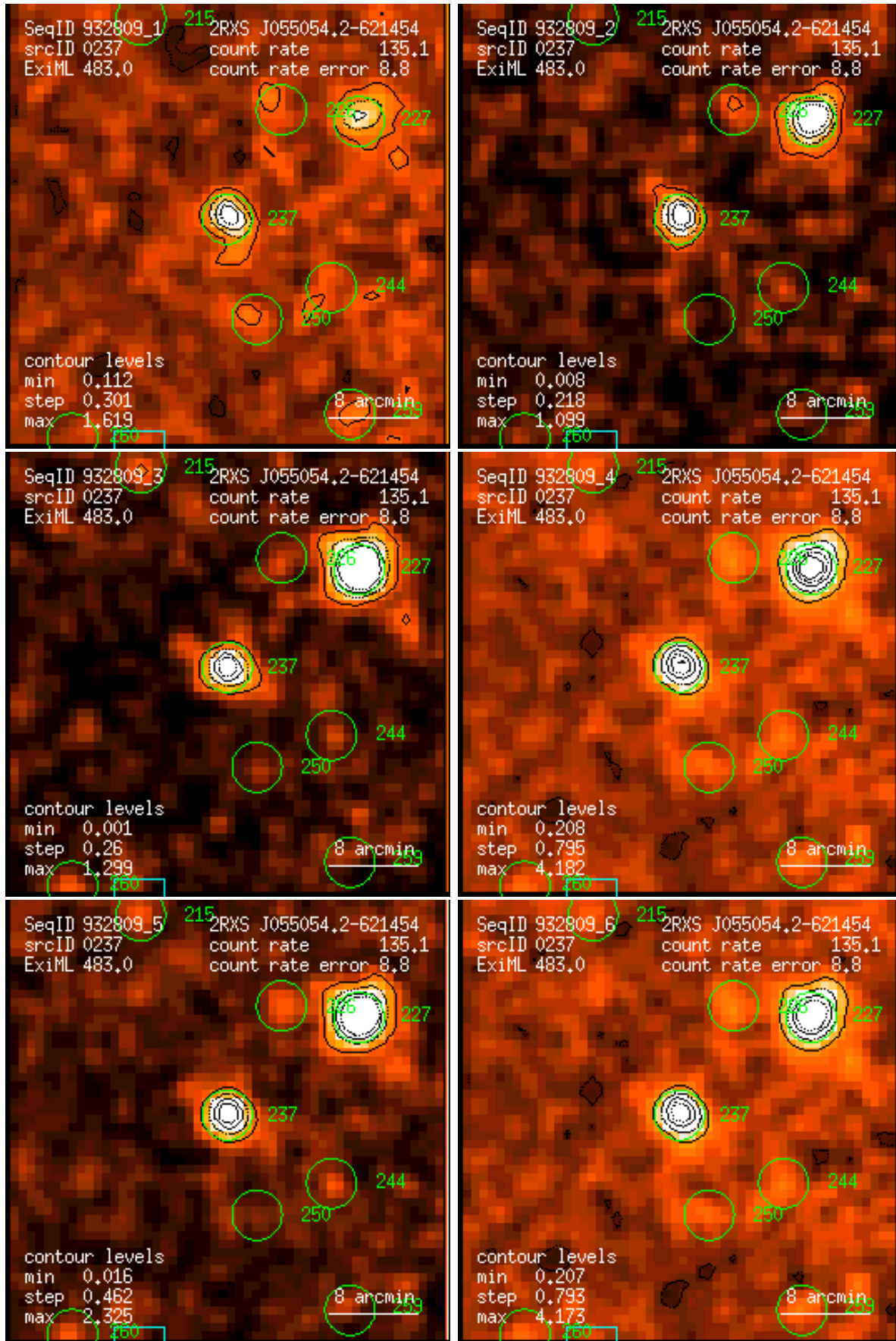
Figure 237: RASS 932809: detection 0237: band rate images, Gaussian filter: (1) PSPC channels 11 – 41, (2) 52 – 90, (3) 91 – 201, (4) 11 – 235, (5) 52 – 201, (6) 11 – 201. Broad band rates in counts/ks. Band rate contour levels in counts/ks/arcmin 2 .
