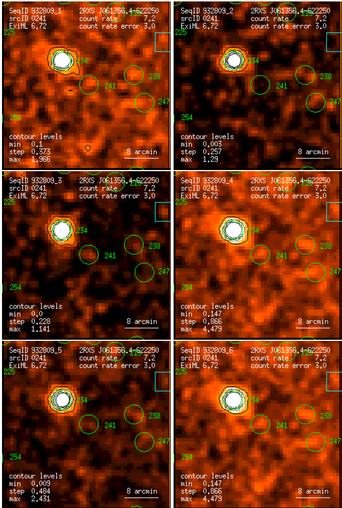
Figure 241: RASS 932809: detection 0241: band rate images, Gaussian filter: (1) PSPC channels 11 – 41, (2) 52 – 90, (3) 91 – 201, (4) 11 – 235, (5) 52 – 201, (6) 11 – 201. Broad band rates in counts/ks. Band rate contour levels in counts/ks/arcmin 2 .
