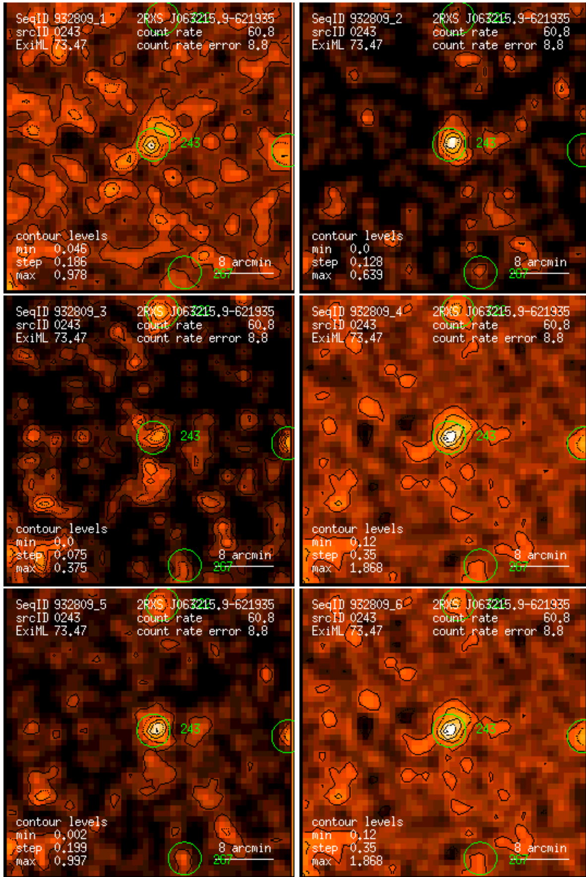
Figure 243: RASS 932809: detection 0243: band rate images, Gaussian filter: (1) PSPC channels 11 – 41, (2) 52 – 90, (3) 91 – 201, (4) 11 – 235, (5) 52 – 201, (6) 11 – 201. Broad band rates in counts/ks. Band rate contour levels in counts/ks/arcmin 2 .
