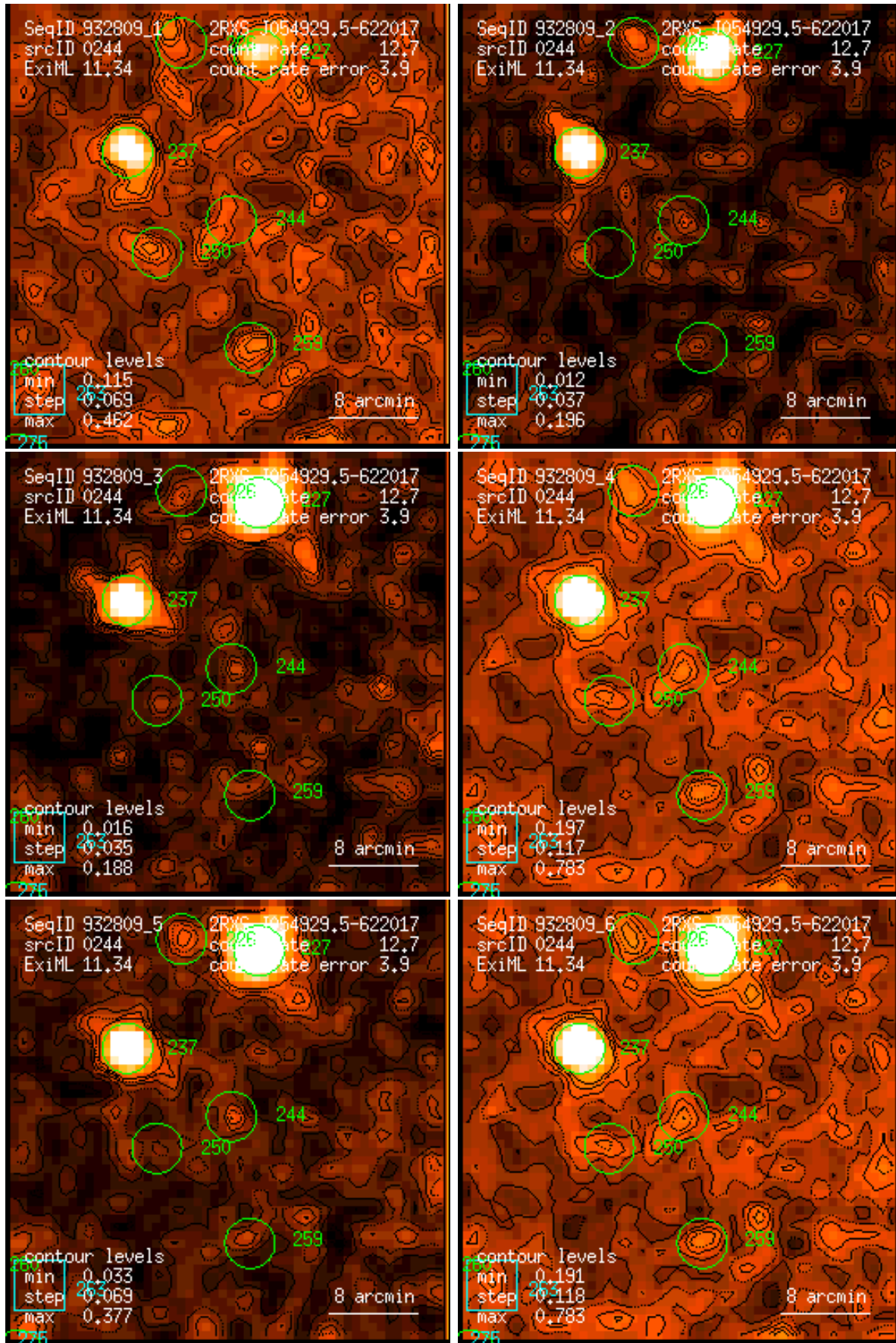
Figure 244: RASS 932809: detection 0244: band rate images, Gaussian filter: (1) PSPC channels 11 – 41, (2) 52 – 90, (3) 91 – 201, (4) 11 – 235, (5) 52 – 201, (6) 11 – 201. Broad band rates in counts/ks. Band rate contour levels in counts/ks/arcmin 2 .
