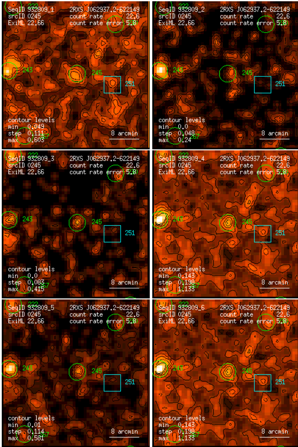
Figure 245: RASS 932809: detection 0245: band rate images, Gaussian filter: (1) PSPC channels 11 – 41, (2) 52 – 90, (3) 91 – 201, (4) 11 – 235, (5) 52 – 201, (6) 11 – 201. Broad band rates in counts/ks. Band rate contour levels in counts/ks/arcmin 2 .
