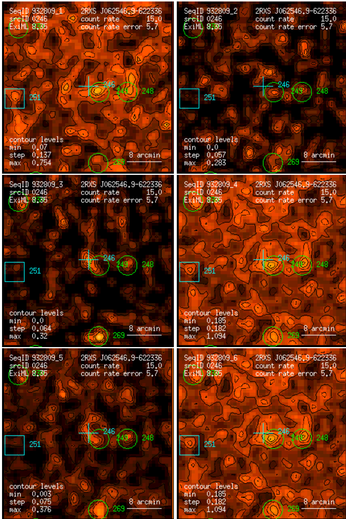
Figure 246: RASS 932809: detection 0246: band rate images, Gaussian filter: (1) PSPC channels 11 – 41, (2) 52 – 90, (3) 91 – 201, (4) 11 – 235, (5) 52 – 201, (6) 11 – 201. Broad band rates in counts/ks. Band rate contour levels in counts/ks/arcmin 2 .
