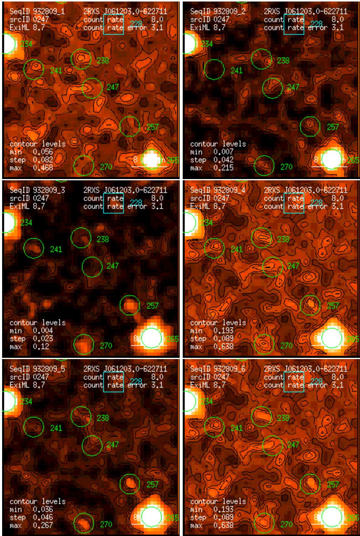
Figure 247: RASS 932809: detection 0247: band rate images, Gaussian filter: (1) PSPC channels 11 – 41, (2) 52 – 90, (3) 91 – 201, (4) 11 – 235, (5) 52 – 201, (6) 11 – 201. Broad band rates in counts/ks. Band rate contour levels in counts/ks/arcmin 2 .
