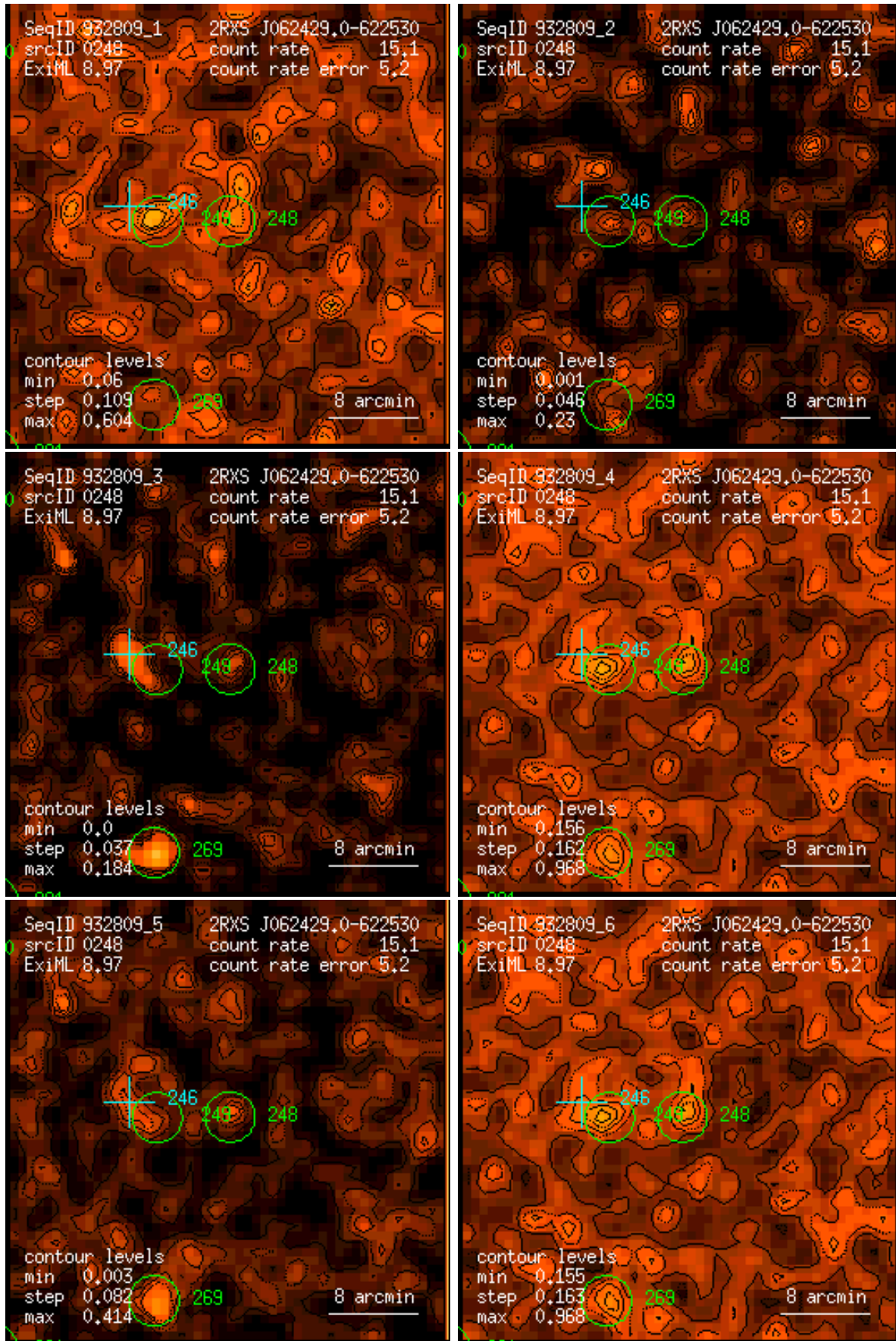
Figure 248: RASS 932809: detection 0248: band rate images, Gaussian filter: (1) PSPC channels 11 – 41, (2) 52 – 90, (3) 91 – 201, (4) 11 – 235, (5) 52 – 201, (6) 11 – 201. Broad band rates in counts/ks. Band rate contour levels in counts/ks/arcmin 2 .
