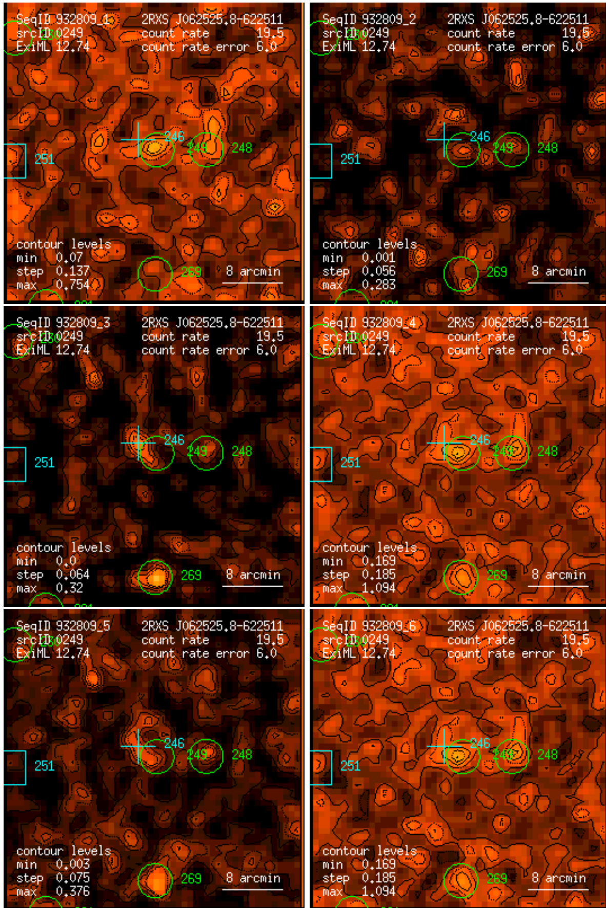
Figure 249: RASS 932809: detection 0249: band rate images, Gaussian filter: (1) PSPC channels 11 – 41, (2) 52 – 90, (3) 91 – 201, (4) 11 – 235, (5) 52 – 201, (6) 11 – 201. Broad band rates in counts/ks. Band rate contour levels in counts/ks/arcmin 2 .
