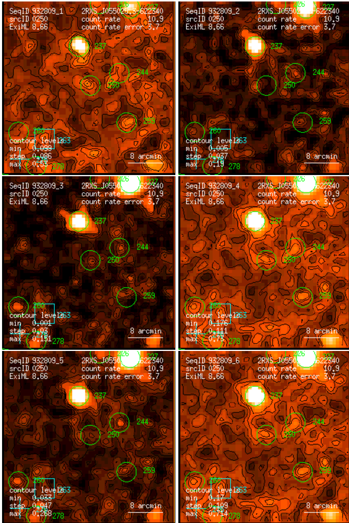
Figure 250: RASS 932809: detection 0250: band rate images, Gaussian filter: (1) PSPC channels 11 – 41, (2) 52 – 90, (3) 91 – 201, (4) 11 – 235, (5) 52 – 201, (6) 11 – 201. Broad band rates in counts/ks. Band rate contour levels in counts/ks/arcmin 2 .
