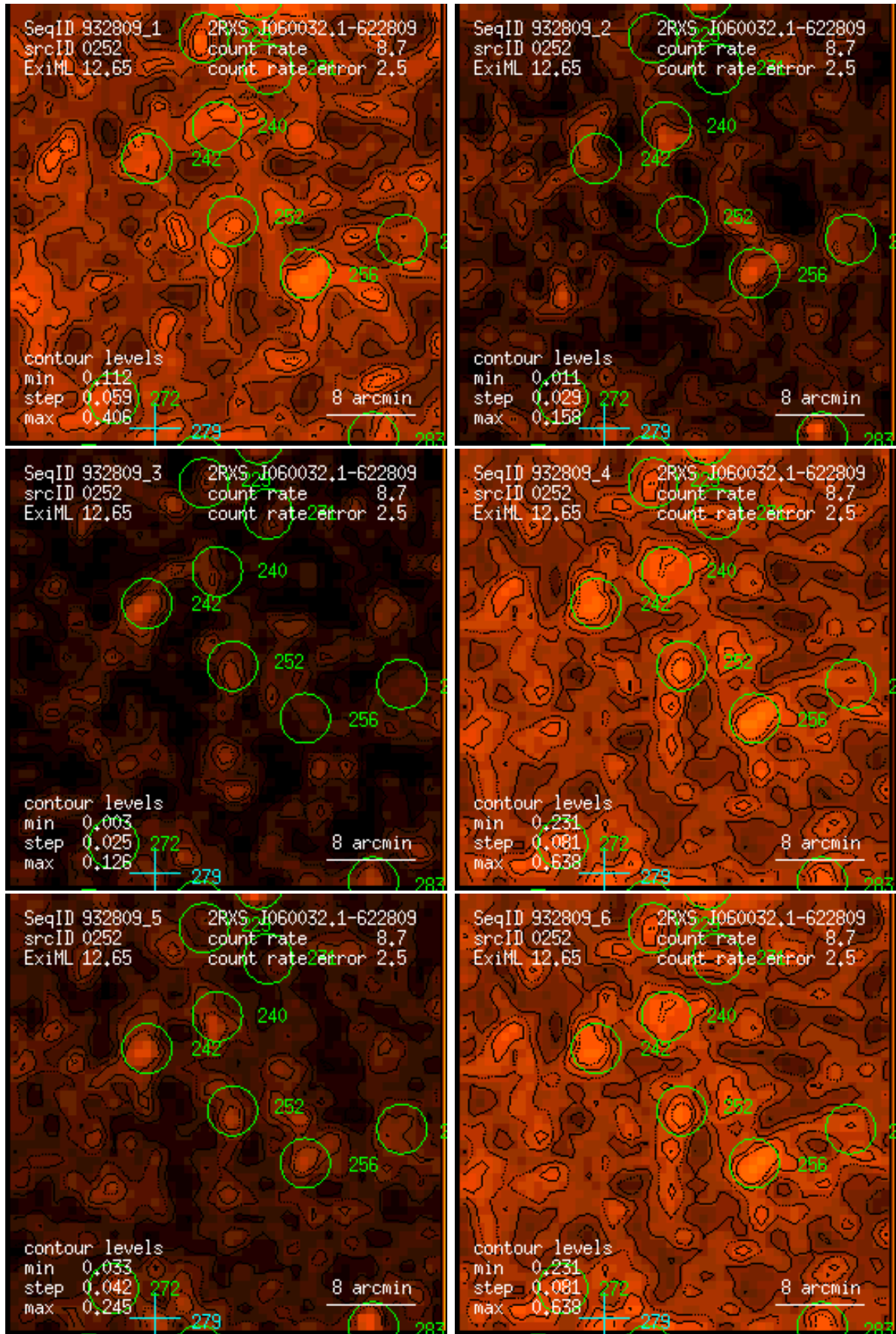
Figure 252: RASS 932809: detection 0252: band rate images, Gaussian filter: (1) PSPC channels 11 – 41, (2) 52 – 90, (3) 91 – 201, (4) 11 – 235, (5) 52 – 201, (6) 11 – 201. Broad band rates in counts/ks. Band rate contour levels in counts/ks/arcmin 2 .
