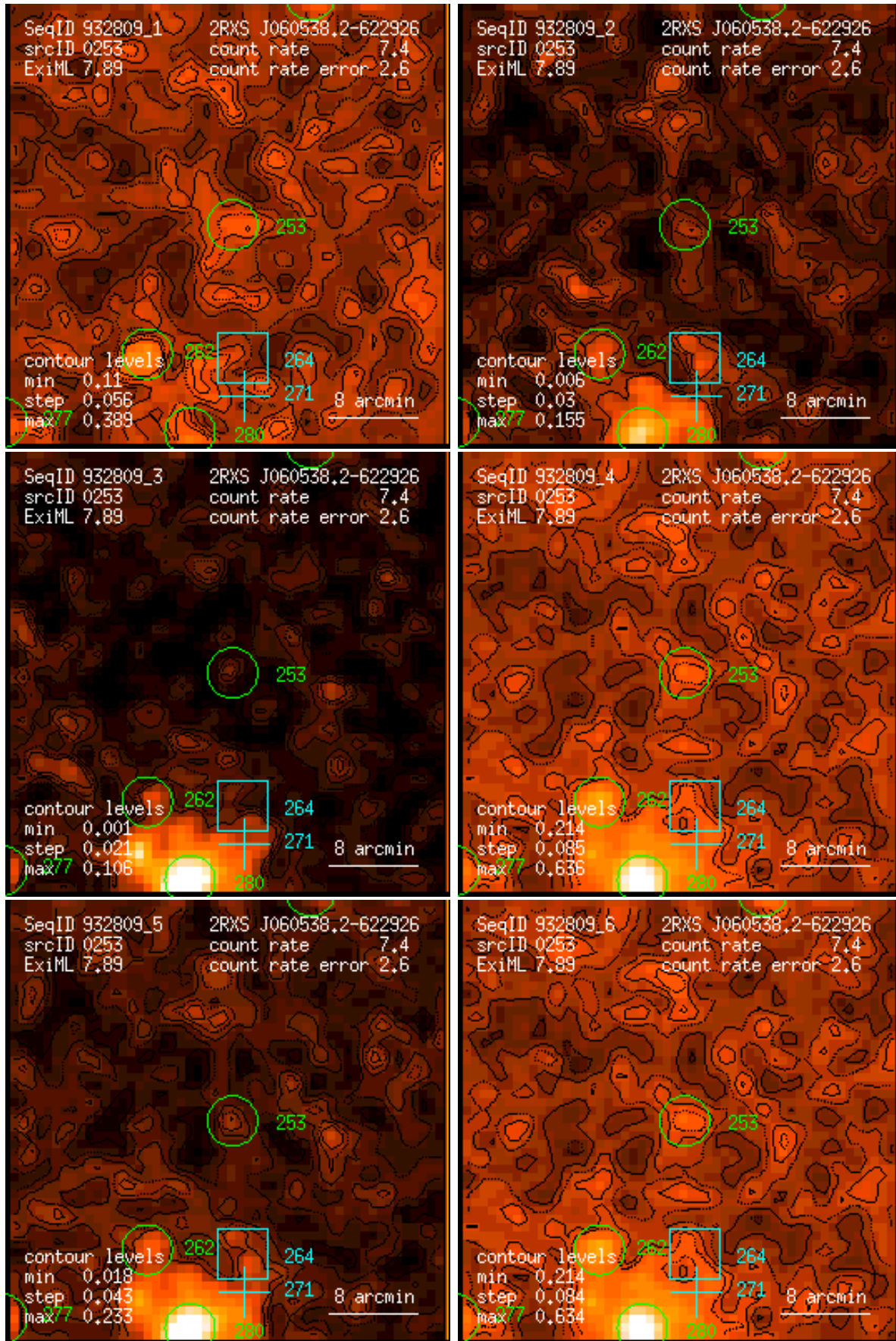
Figure 253: RASS 932809: detection 0253: band rate images, Gaussian filter: (1) PSPC channels 11 – 41, (2) 52 – 90, (3) 91 – 201, (4) 11 – 235, (5) 52 – 201, (6) 11 – 201. Broad band rates in counts/ks. Band rate contour levels in counts/ks/arcmin 2 .
