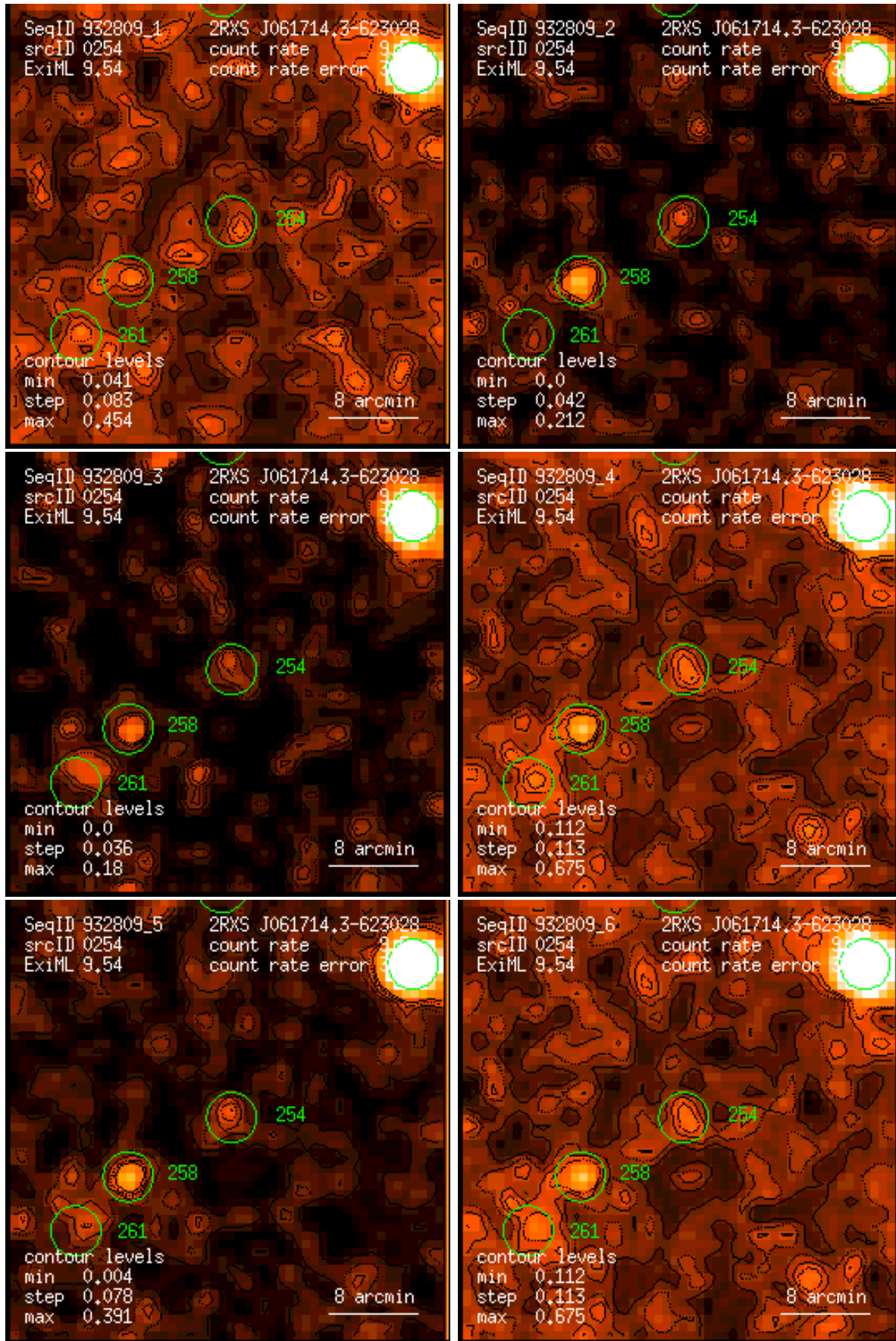
Figure 254: RASS 932809: detection 0254: band rate images, Gaussian filter: (1) PSPC channels 11 – 41, (2) 52 – 90, (3) 91 – 201, (4) 11 – 235, (5) 52 – 201, (6) 11 – 201. Broad band rates in counts/ks. Band rate contour levels in counts/ks/arcmin 2 .
