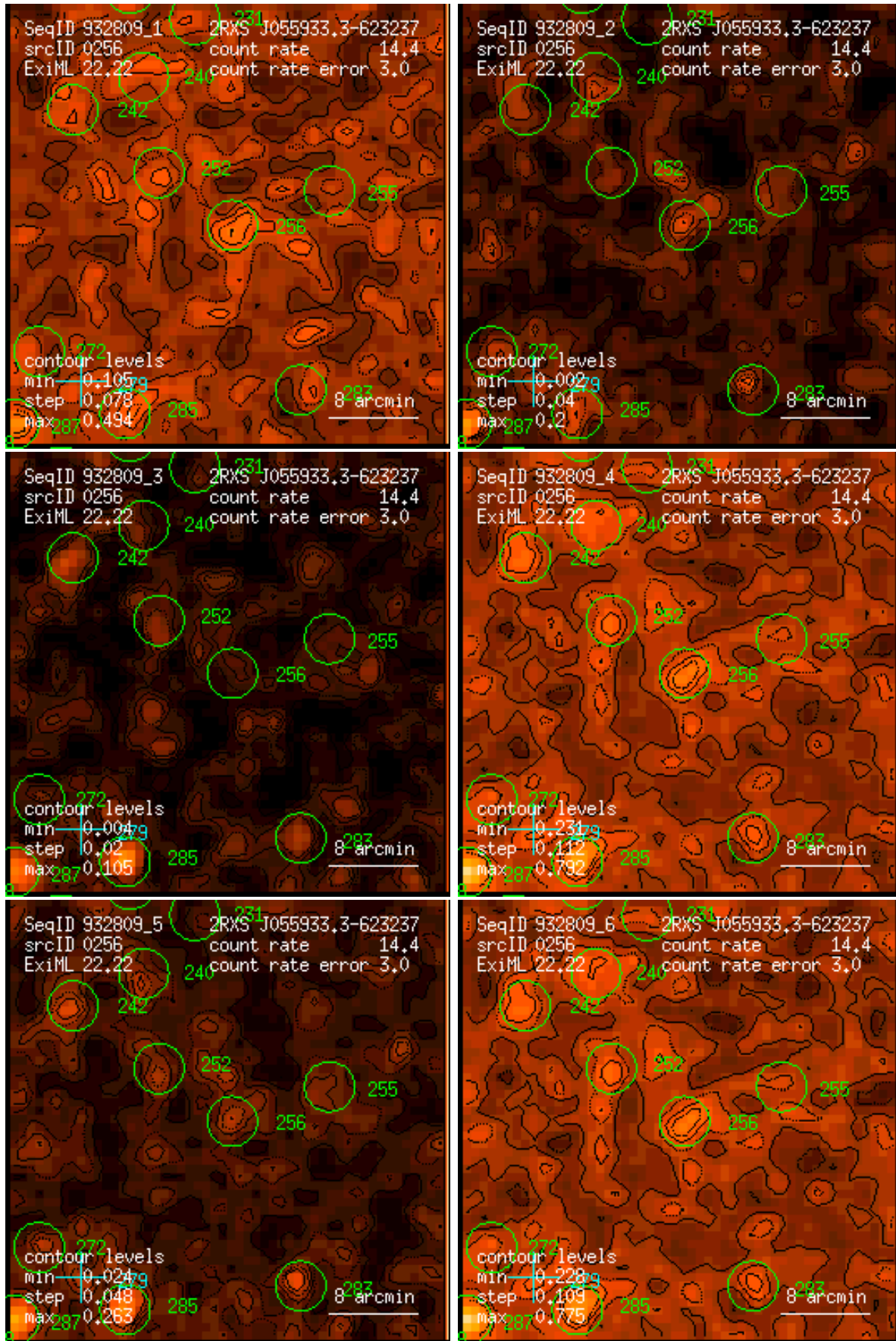
Figure 256: RASS 932809: detection 0256: band rate images, Gaussian filter: (1) PSPC channels 11 – 41, (2) 52 – 90, (3) 91 – 201, (4) 11 – 235, (5) 52 – 201, (6) 11 – 201. Broad band rates in counts/ks. Band rate contour levels in counts/ks/arcmin 2 .
