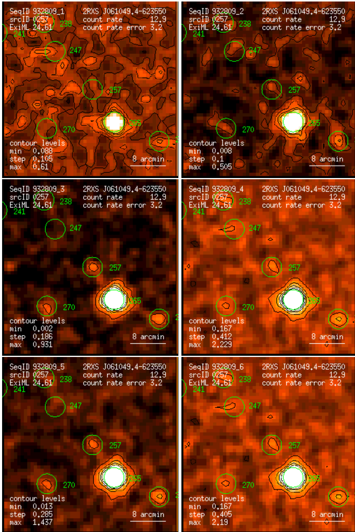
Figure 257: RASS 932809: detection 0257: band rate images, Gaussian filter: (1) PSPC channels 11 – 41, (2) 52 – 90, (3) 91 – 201, (4) 11 – 235, (5) 52 – 201, (6) 11 – 201. Broad band rates in counts/ks. Band rate contour levels in counts/ks/arcmin 2 .
