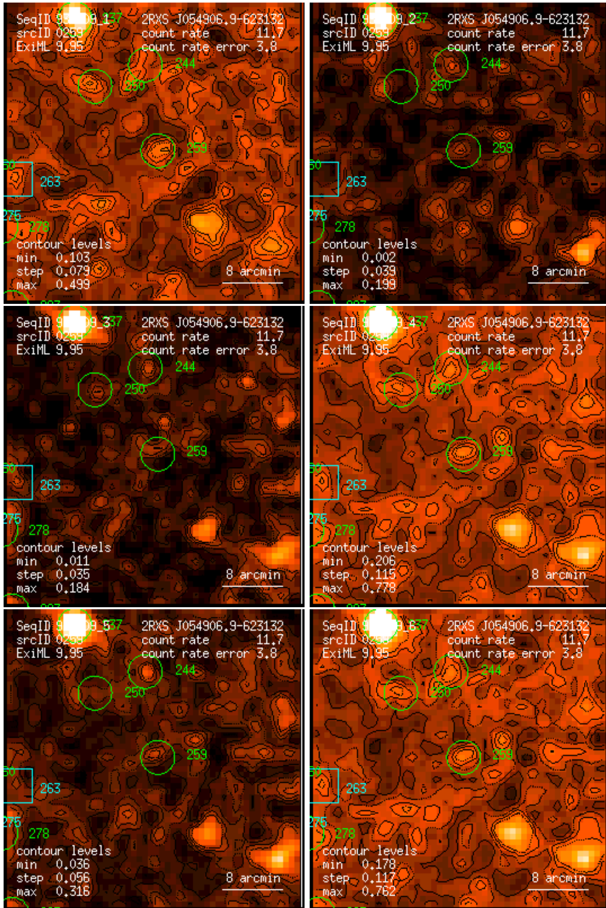
Figure 259: RASS 932809: detection 0259: band rate images, Gaussian filter: (1) PSPC channels 11 – 41, (2) 52 – 90, (3) 91 – 201, (4) 11 – 235, (5) 52 – 201, (6) 11 – 201. Broad band rates in counts/ks. Band rate contour levels in counts/ks/arcmin 2 .
