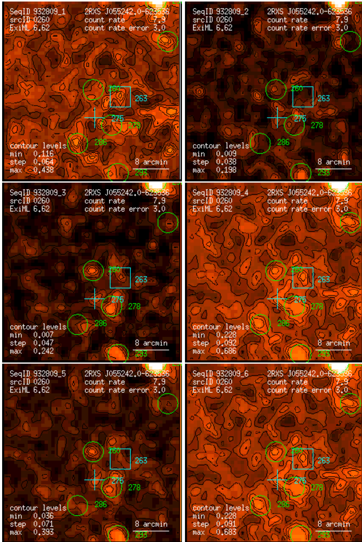
Figure 260: RASS 932809: detection 0260: band rate images, Gaussian filter: (1) PSPC channels 11 – 41, (2) 52 – 90, (3) 91 – 201, (4) 11 – 235, (5) 52 – 201, (6) 11 – 201. Broad band rates in counts/ks. Band rate contour levels in counts/ks/arcmin 2 .
