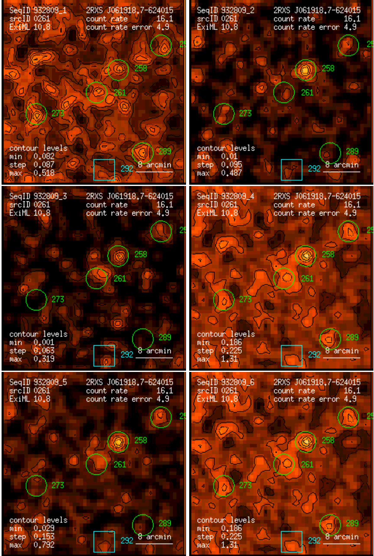
Figure 261: RASS 932809: detection 0261: band rate images, Gaussian filter: (1) PSPC channels 11 – 41, (2) 52 – 90, (3) 91 – 201, (4) 11 – 235, (5) 52 – 201, (6) 11 – 201. Broad band rates in counts/ks. Band rate contour levels in counts/ks/arcmin 2 .
