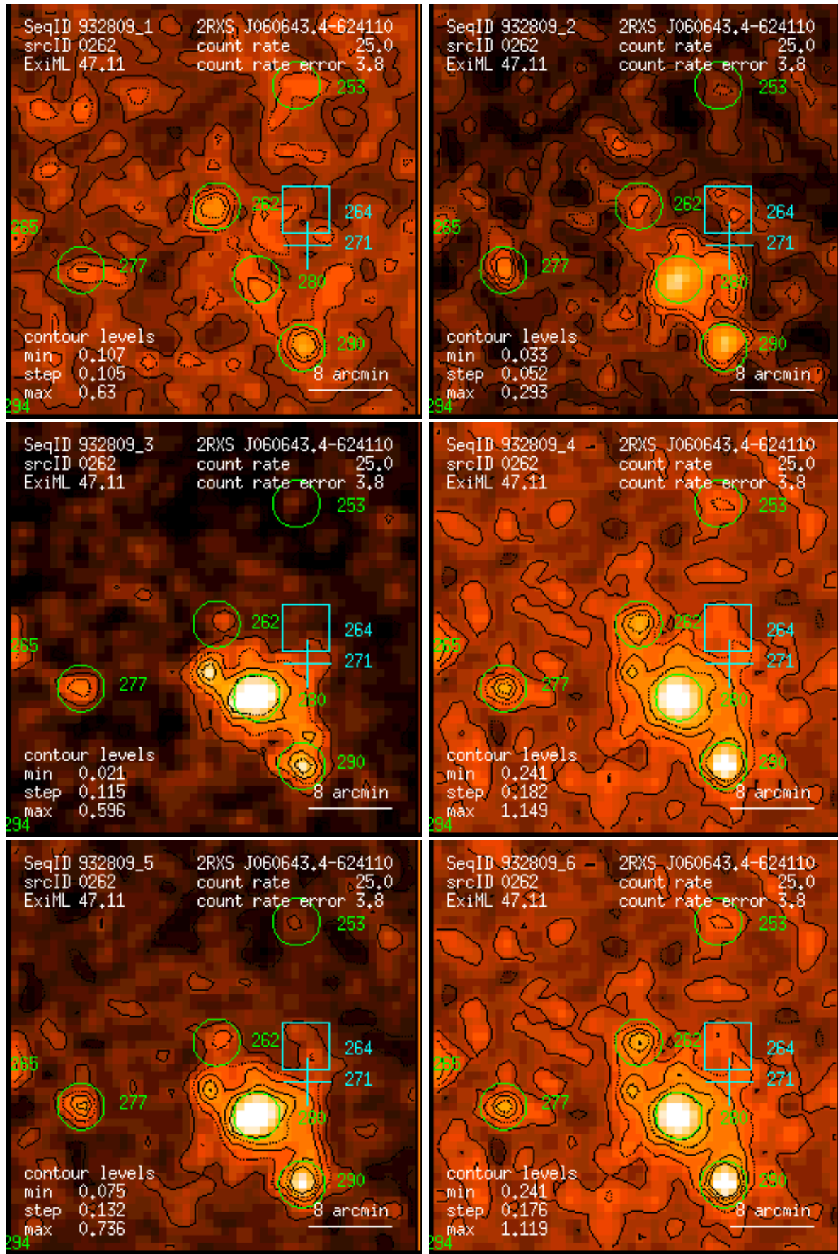
Figure 262: RASS 932809: detection 0262: band rate images, Gaussian filter: (1) PSPC channels 11 – 41, (2) 52 – 90, (3) 91 – 201, (4) 11 – 235, (5) 52 – 201, (6) 11 – 201. Broad band rates in counts/ks. Band rate contour levels in counts/ks/arcmin 2 .
