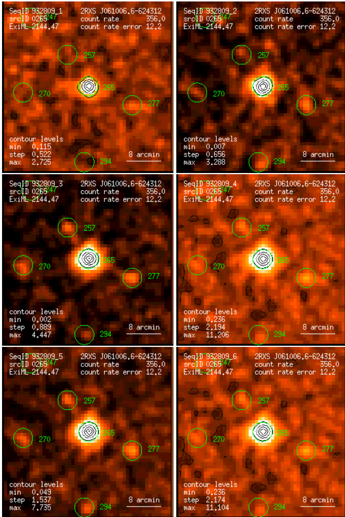
Figure 265: RASS 932809: detection 0265: band rate images, Gaussian filter: (1) PSPC channels 11 – 41, (2) 52 – 90, (3) 91 – 201, (4) 11 – 235, (5) 52 – 201, (6) 11 – 201. Broad band rates in counts/ks. Band rate contour levels in counts/ks/arcmin 2 .
