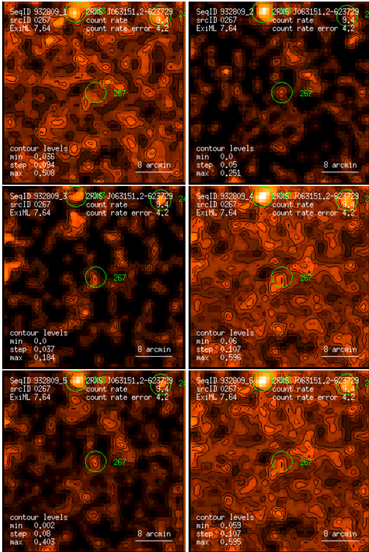
Figure 267: RASS 932809: detection 0267: band rate images, Gaussian filter: (1) PSPC channels 11 – 41, (2) 52 – 90, (3) 91 – 201, (4) 11 – 235, (5) 52 – 201, (6) 11 – 201. Broad band rates in counts/ks. Band rate contour levels in counts/ks/arcmin 2 .
