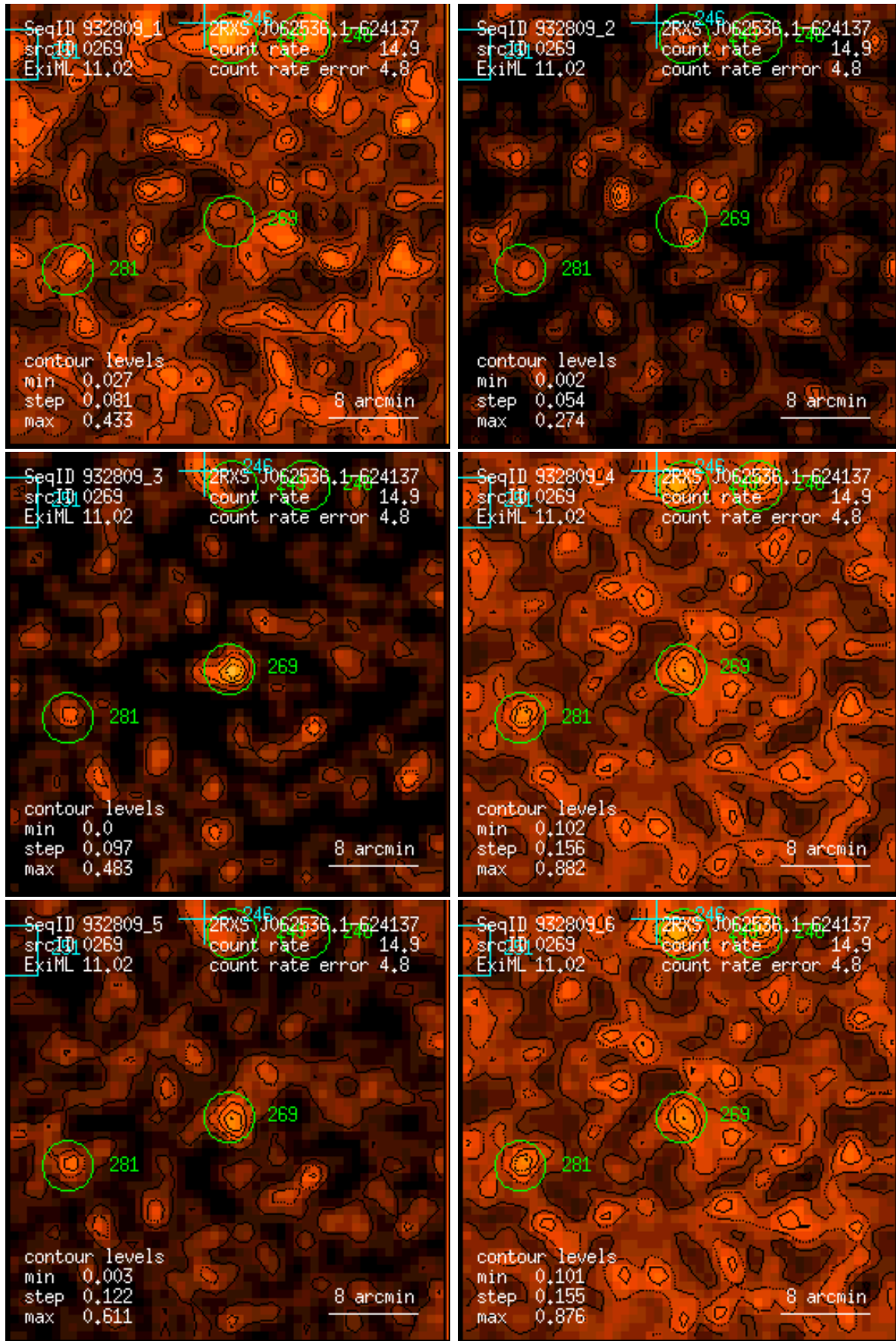
Figure 269: RASS 932809: detection 0269: band rate images, Gaussian filter: (1) PSPC channels 11 – 41, (2) 52 – 90, (3) 91 – 201, (4) 11 – 235, (5) 52 – 201, (6) 11 – 201. Broad band rates in counts/ks. Band rate contour levels in counts/ks/arcmin 2 .
