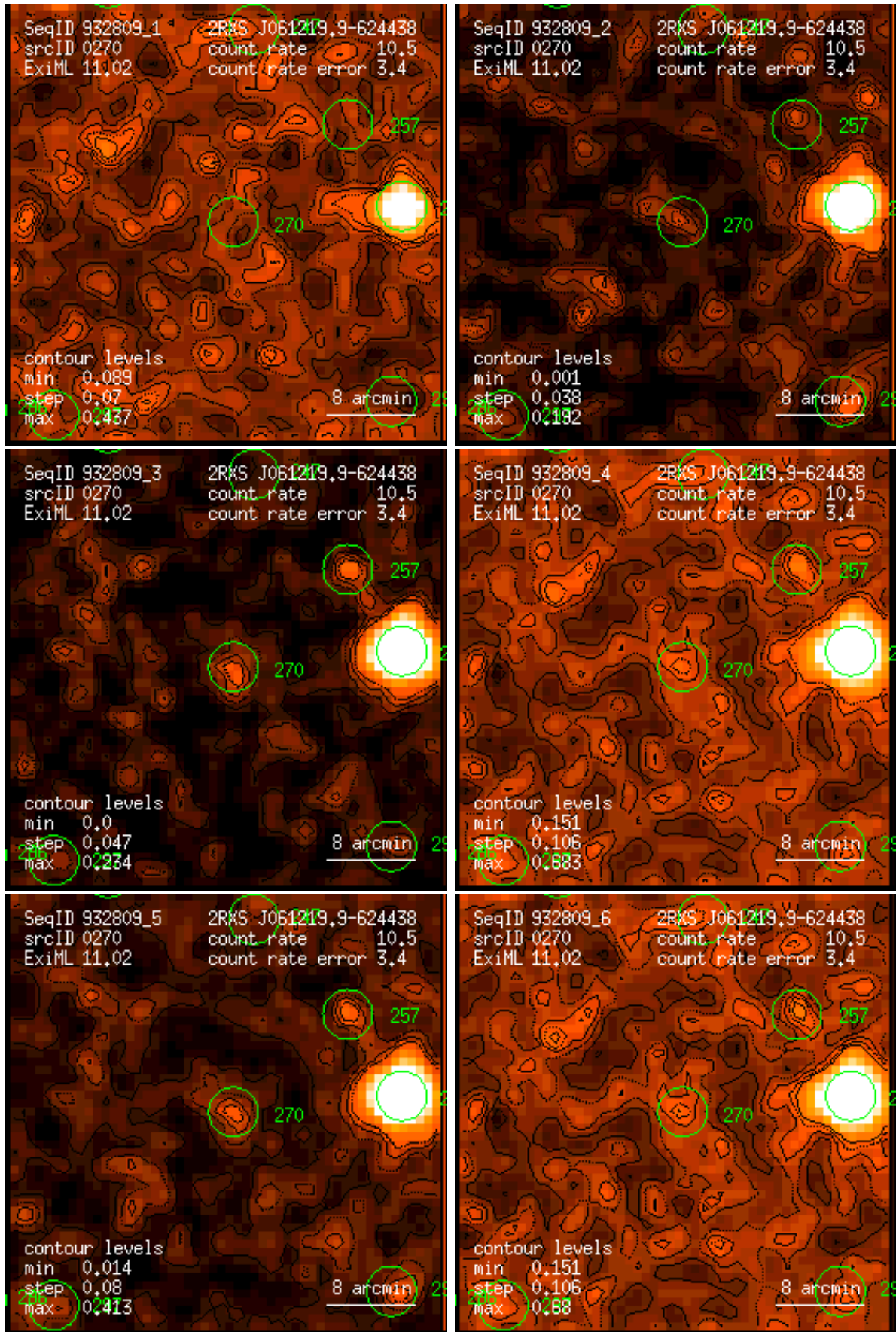
Figure 270: RASS 932809: detection 0270: band rate images, Gaussian filter: (1) PSPC channels 11 – 41, (2) 52 – 90, (3) 91 – 201, (4) 11 – 235, (5) 52 – 201, (6) 11 – 201. Broad band rates in counts/ks. Band rate contour levels in counts/ks/arcmin 2 .
