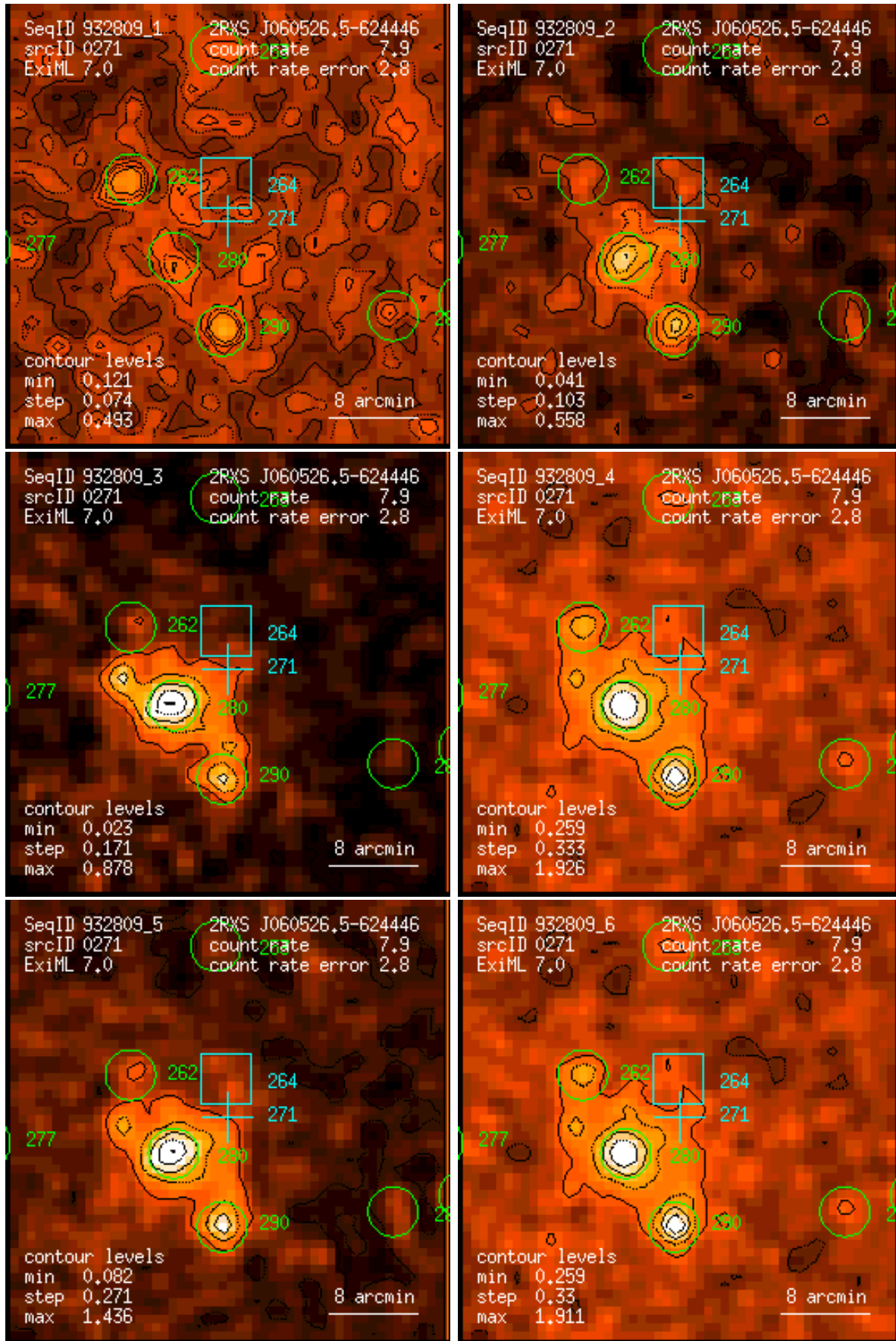
Figure 271: RASS 932809: detection 0271: band rate images, Gaussian filter: (1) PSPC channels 11 – 41, (2) 52 – 90, (3) 91 – 201, (4) 11 – 235, (5) 52 – 201, (6) 11 – 201. Broad band rates in counts/ks. Band rate contour levels in counts/ks/arcmin 2 .
