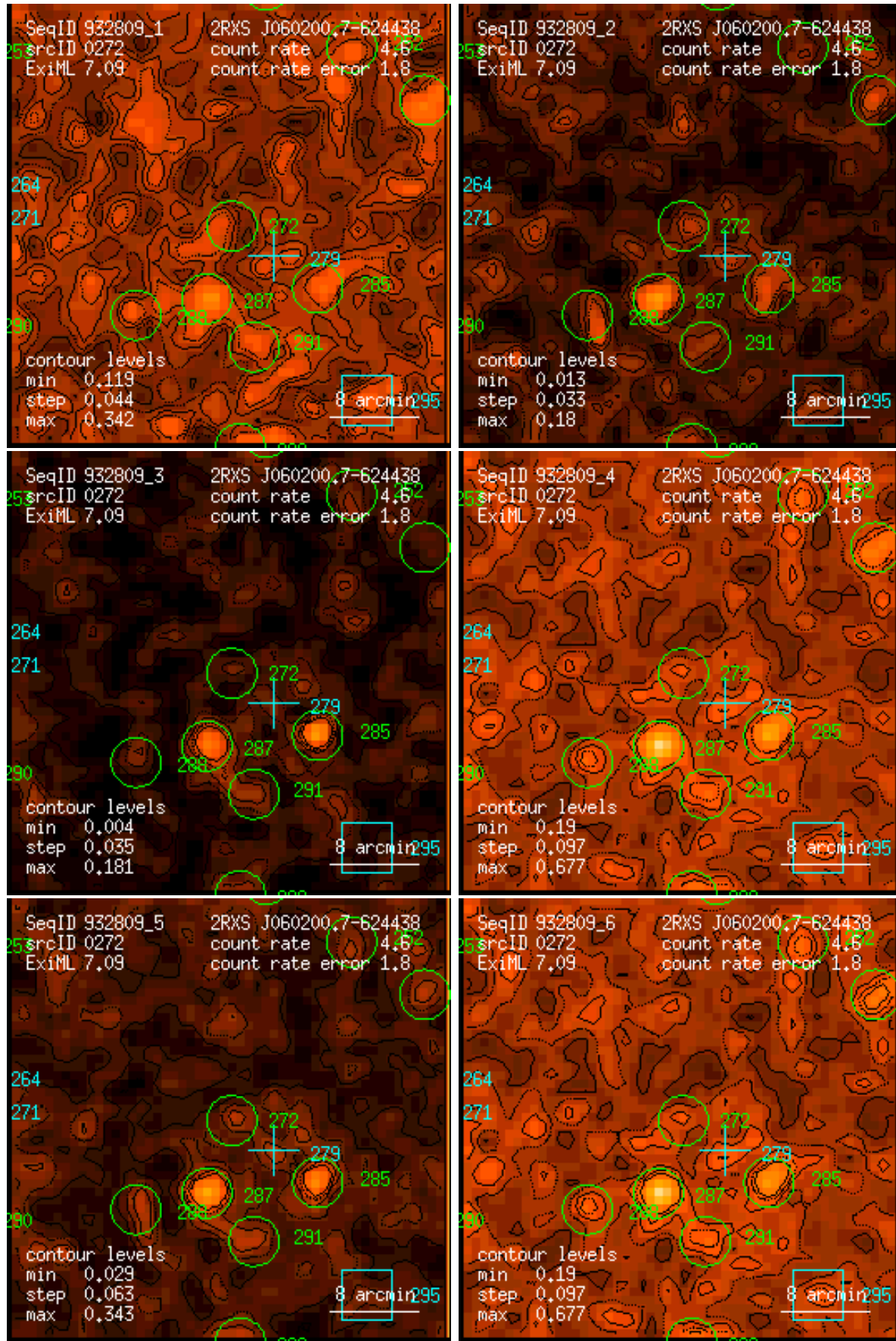
Figure 272: RASS 932809: detection 0272: band rate images, Gaussian filter: (1) PSPC channels 11 – 41, (2) 52 – 90, (3) 91 – 201, (4) 11 – 235, (5) 52 – 201, (6) 11 – 201. Broad band rates in counts/ks. Band rate contour levels in counts/ks/arcmin 2 .
