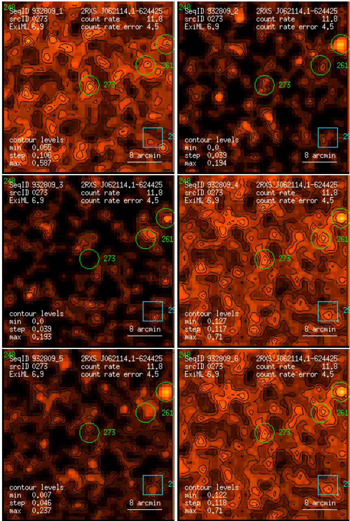
Figure 273: RASS 932809: detection 0273: band rate images, Gaussian filter: (1) PSPC channels 11 – 41, (2) 52 – 90, (3) 91 – 201, (4) 11 – 235, (5) 52 – 201, (6) 11 – 201. Broad band rates in counts/ks. Band rate contour levels in counts/ks/arcmin 2 .
