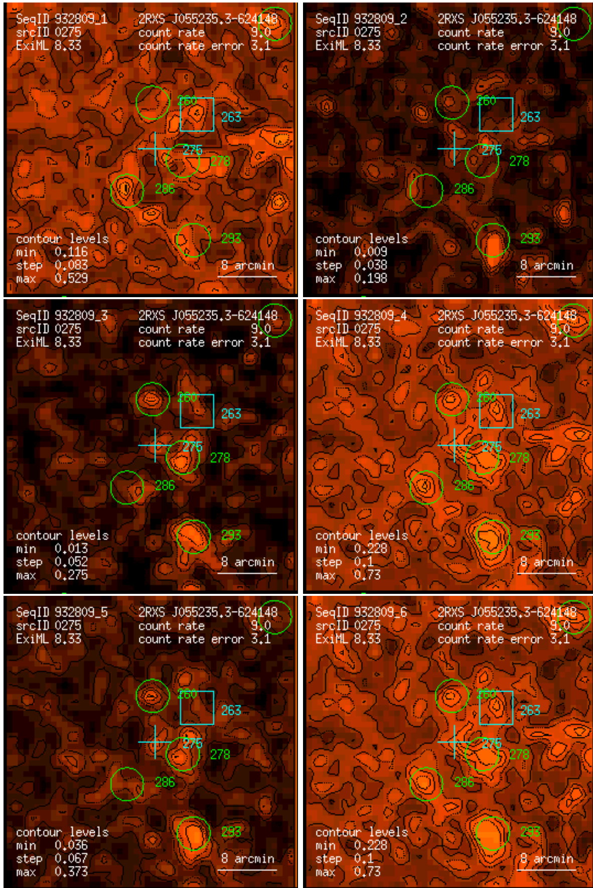
Figure 275: RASS 932809: detection 0275: band rate images, Gaussian filter: (1) PSPC channels 11 – 41, (2) 52 – 90, (3) 91 – 201, (4) 11 – 235, (5) 52 – 201, (6) 11 – 201. Broad band rates in counts/ks. Band rate contour levels in counts/ks/arcmin 2 .
