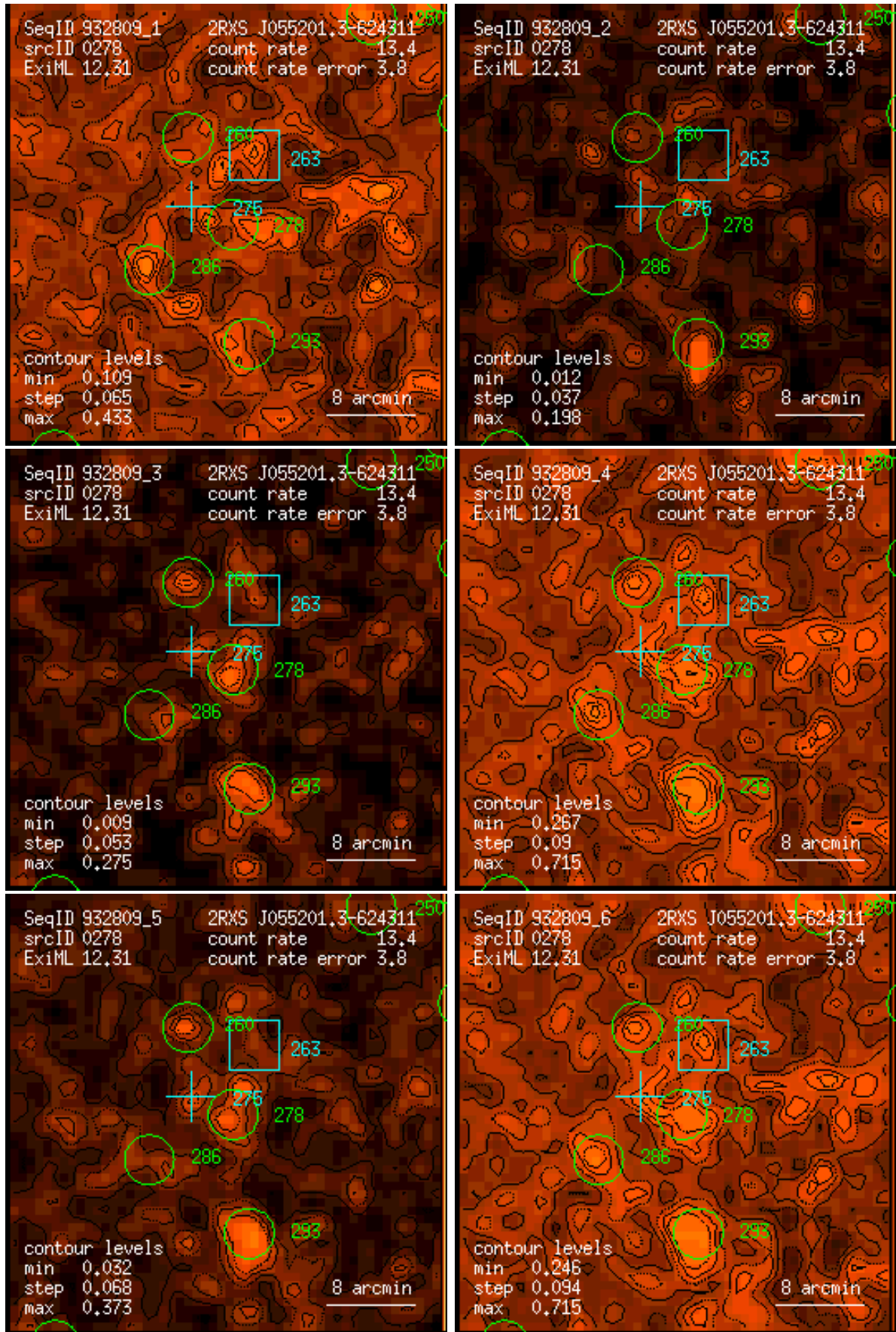
Figure 278: RASS 932809: detection 0278: band rate images, Gaussian filter: (1) PSPC channels 11 – 41, (2) 52 – 90, (3) 91 – 201, (4) 11 – 235, (5) 52 – 201, (6) 11 – 201. Broad band rates in counts/ks. Band rate contour levels in counts/ks/arcmin 2 .
