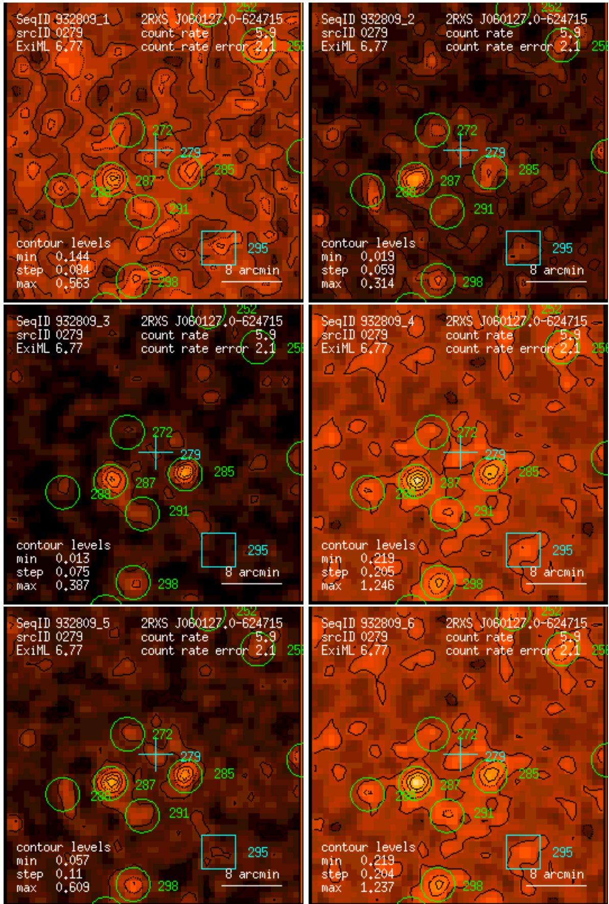
Figure 279: RASS 932809: detection 0279: band rate images, Gaussian filter: (1) PSPC channels 11 – 41, (2) 52 – 90, (3) 91 – 201, (4) 11 – 235, (5) 52 – 201, (6) 11 – 201. Broad band rates in counts/ks. Band rate contour levels in counts/ks/arcmin 2 .
