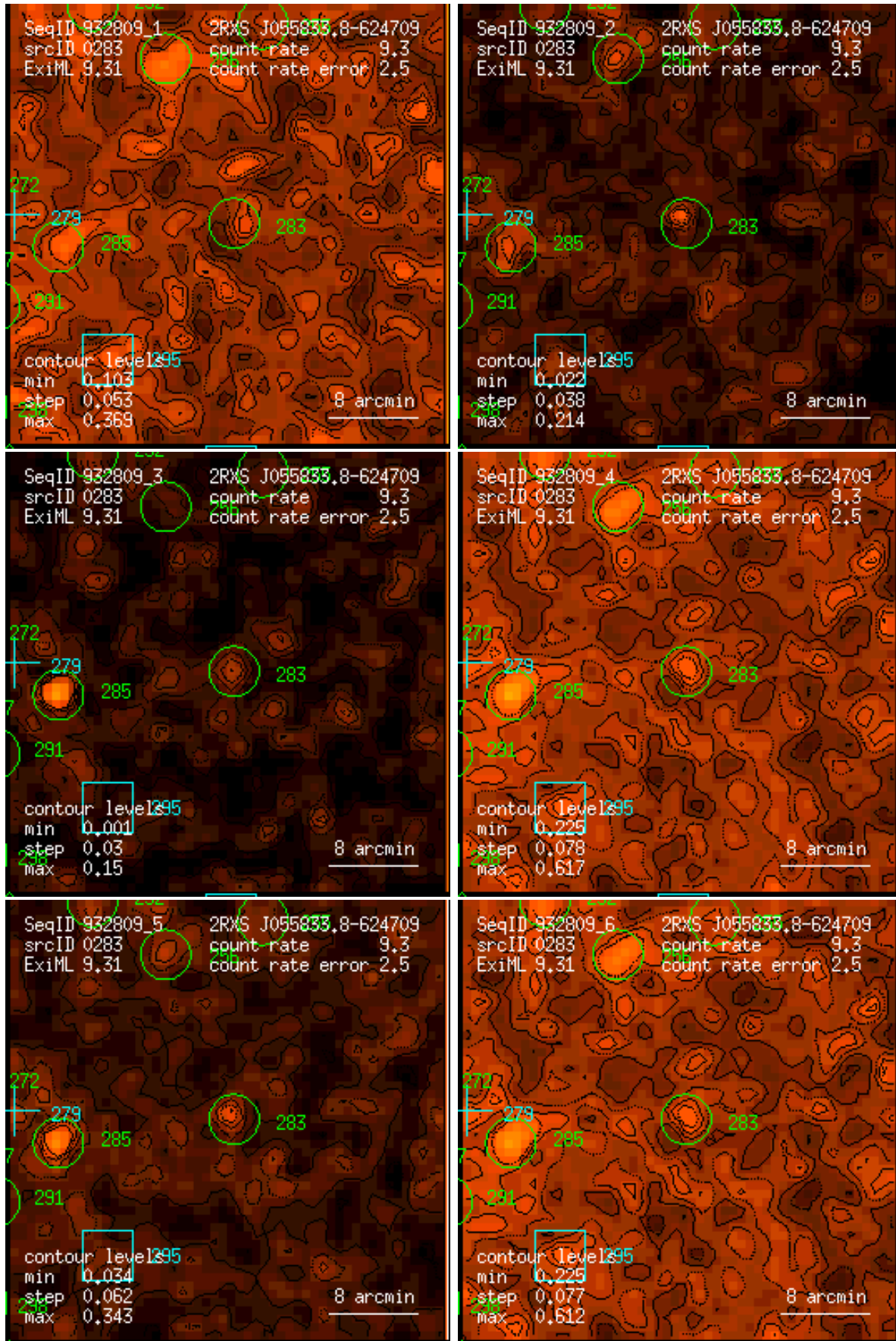
Figure 283: RASS 932809: detection 0283: band rate images, Gaussian filter: (1) PSPC channels 11 – 41, (2) 52 – 90, (3) 91 – 201, (4) 11 – 235, (5) 52 – 201, (6) 11 – 201. Broad band rates in counts/ks. Band rate contour levels in counts/ks/arcmin 2 .
