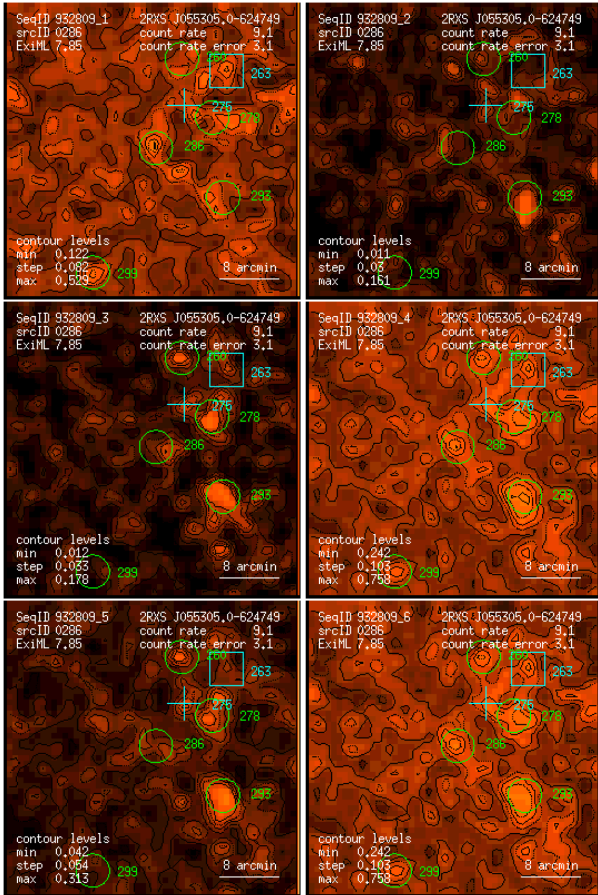
Figure 286: RASS 932809: detection 0286: band rate images, Gaussian filter: (1) PSPC channels 11 – 41, (2) 52 – 90, (3) 91 – 201, (4) 11 – 235, (5) 52 – 201, (6) 11 – 201. Broad band rates in counts/ks. Band rate contour levels in counts/ks/arcmin 2 .
