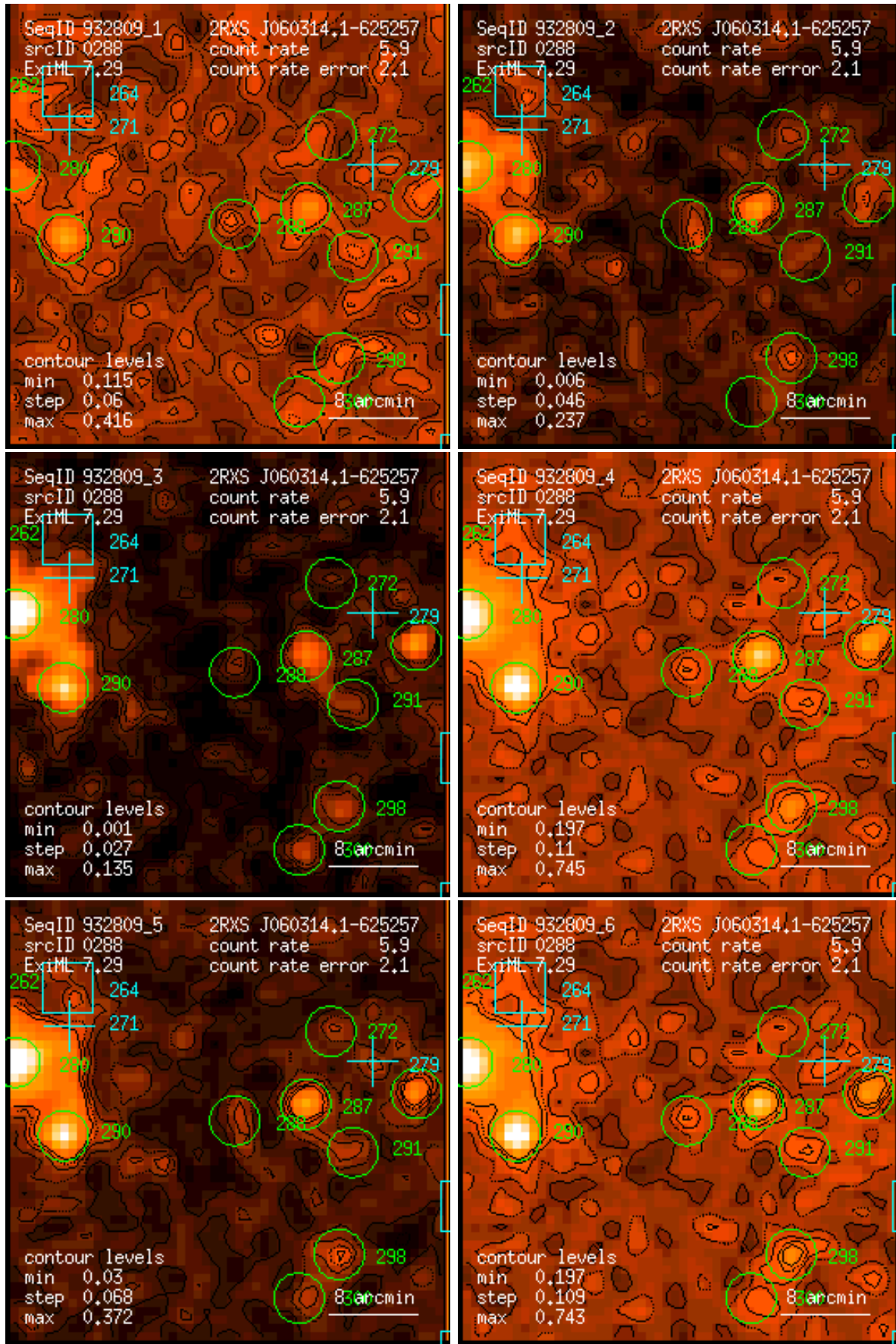
Figure 288: RASS 932809: detection 0288: band rate images, Gaussian filter: (1) PSPC channels 11 – 41, (2) 52 – 90, (3) 91 – 201, (4) 11 – 235, (5) 52 – 201, (6) 11 – 201. Broad band rates in counts/ks. Band rate contour levels in counts/ks/arcmin 2 .
