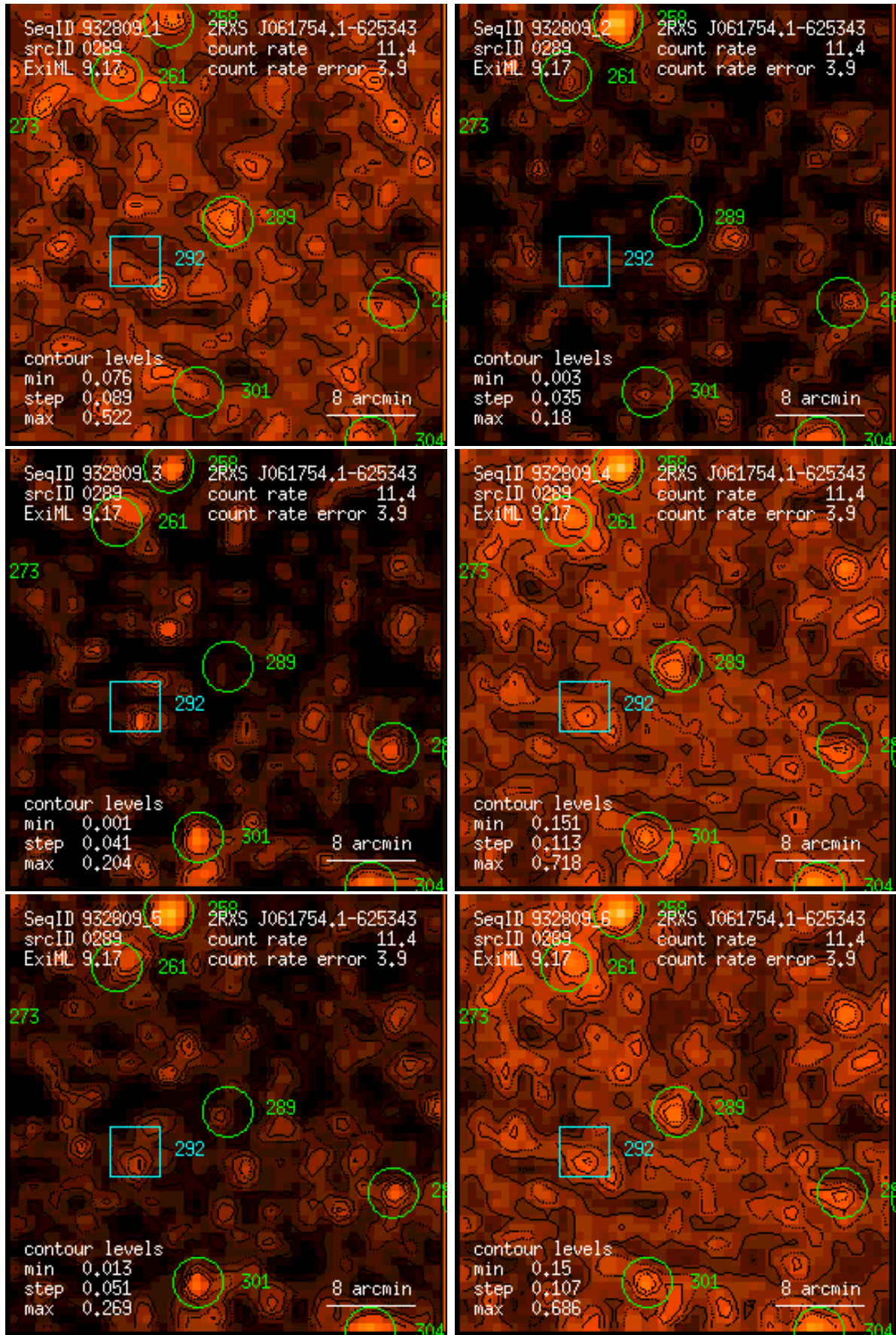
Figure 289: RASS 932809: detection 0289: band rate images, Gaussian filter: (1) PSPC channels 11 – 41, (2) 52 – 90, (3) 91 – 201, (4) 11 – 235, (5) 52 – 201, (6) 11 – 201. Broad band rates in counts/ks. Band rate contour levels in counts/ks/arcmin 2 .
