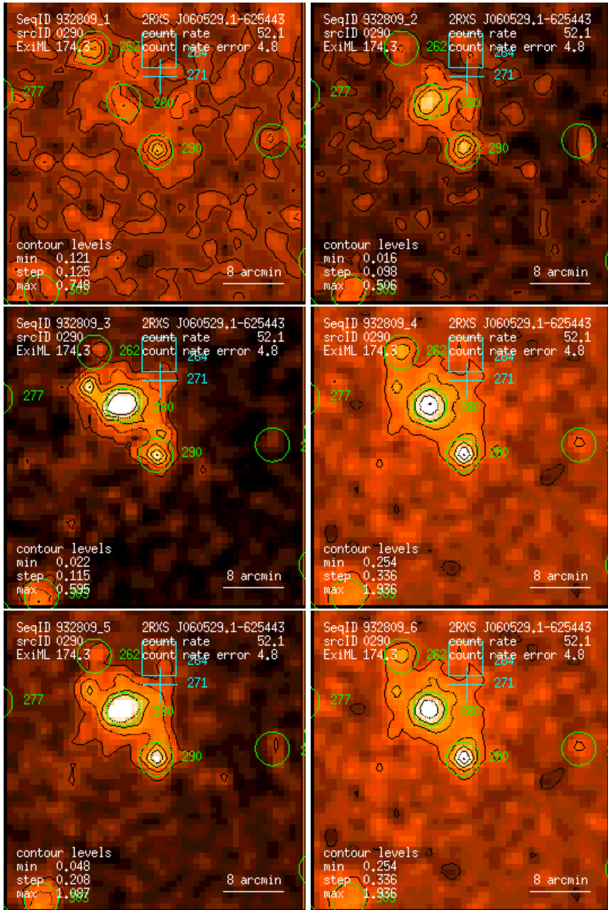
Figure 290: RASS 932809: detection 0290: band rate images, Gaussian filter: (1) PSPC channels 11 – 41, (2) 52 – 90, (3) 91 – 201, (4) 11 – 235, (5) 52 – 201, (6) 11 – 201. Broad band rates in counts/ks. Band rate contour levels in counts/ks/arcmin 2 .
