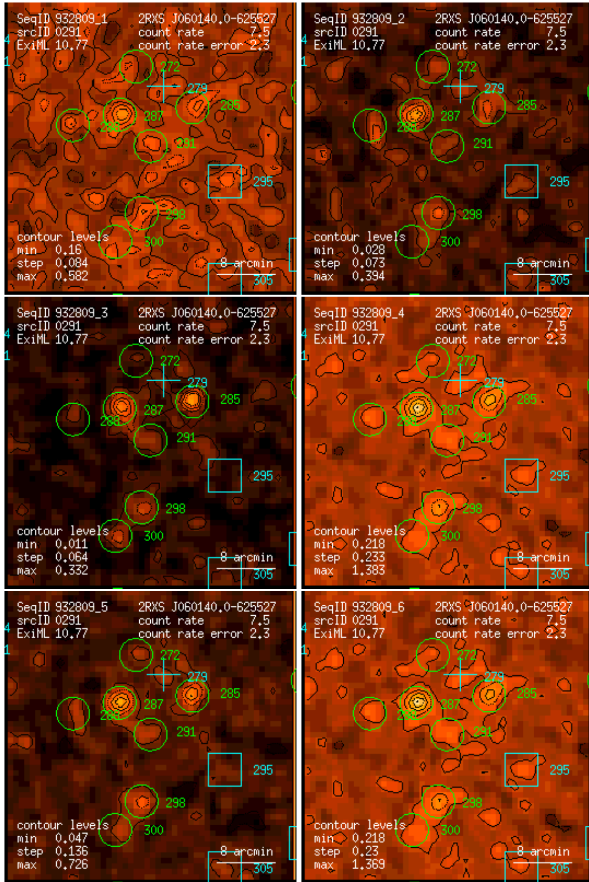
Figure 291: RASS 932809: detection 0291: band rate images, Gaussian filter: (1) PSPC channels 11 – 41, (2) 52 – 90, (3) 91 – 201, (4) 11 – 235, (5) 52 – 201, (6) 11 – 201. Broad band rates in counts/ks. Band rate contour levels in counts/ks/arcmin 2 .
