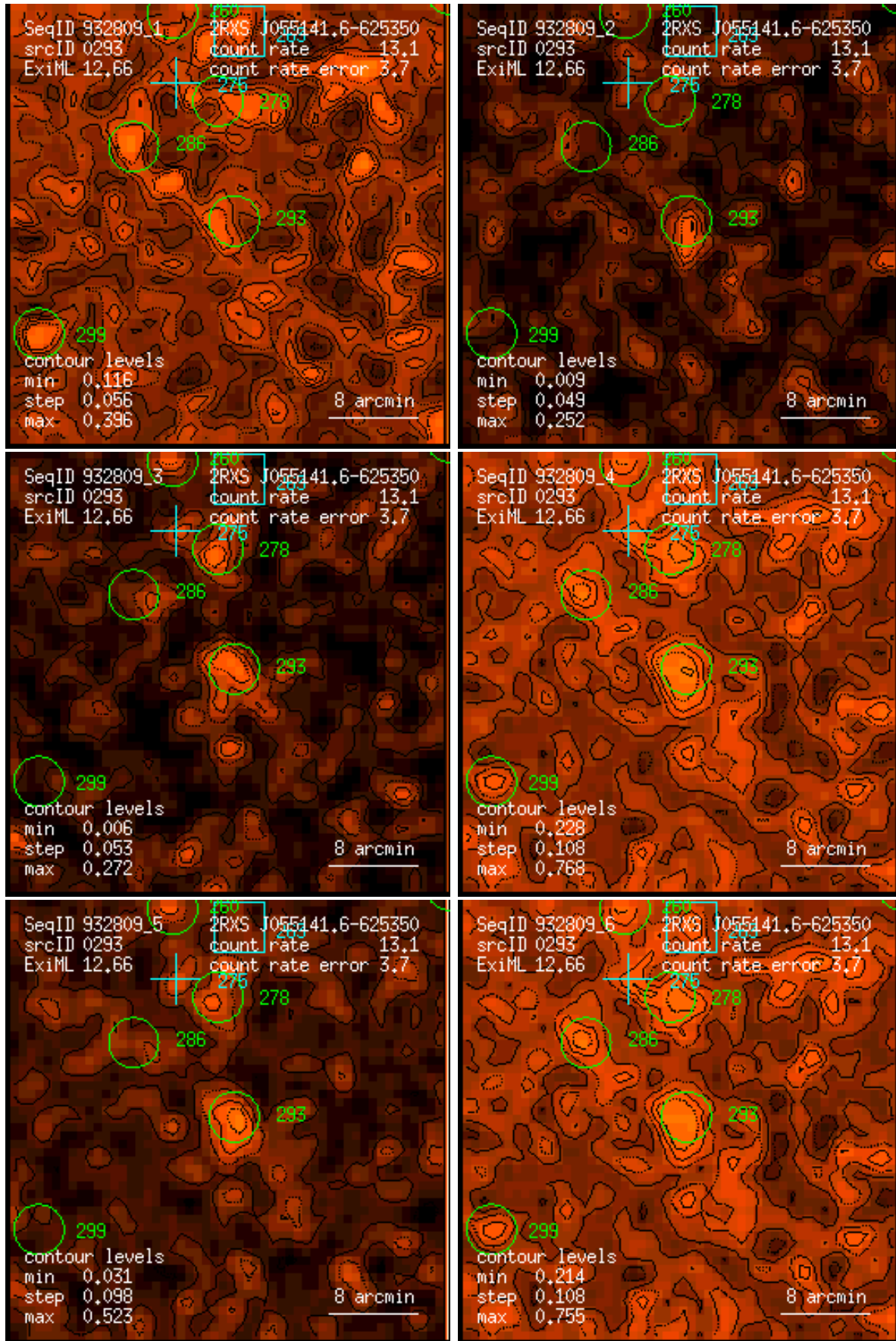
Figure 293: RASS 932809: detection 0293: band rate images, Gaussian filter: (1) PSPC channels 11 – 41, (2) 52 – 90, (3) 91 – 201, (4) 11 – 235, (5) 52 – 201, (6) 11 – 201. Broad band rates in counts/ks. Band rate contour levels in counts/ks/arcmin 2 .
