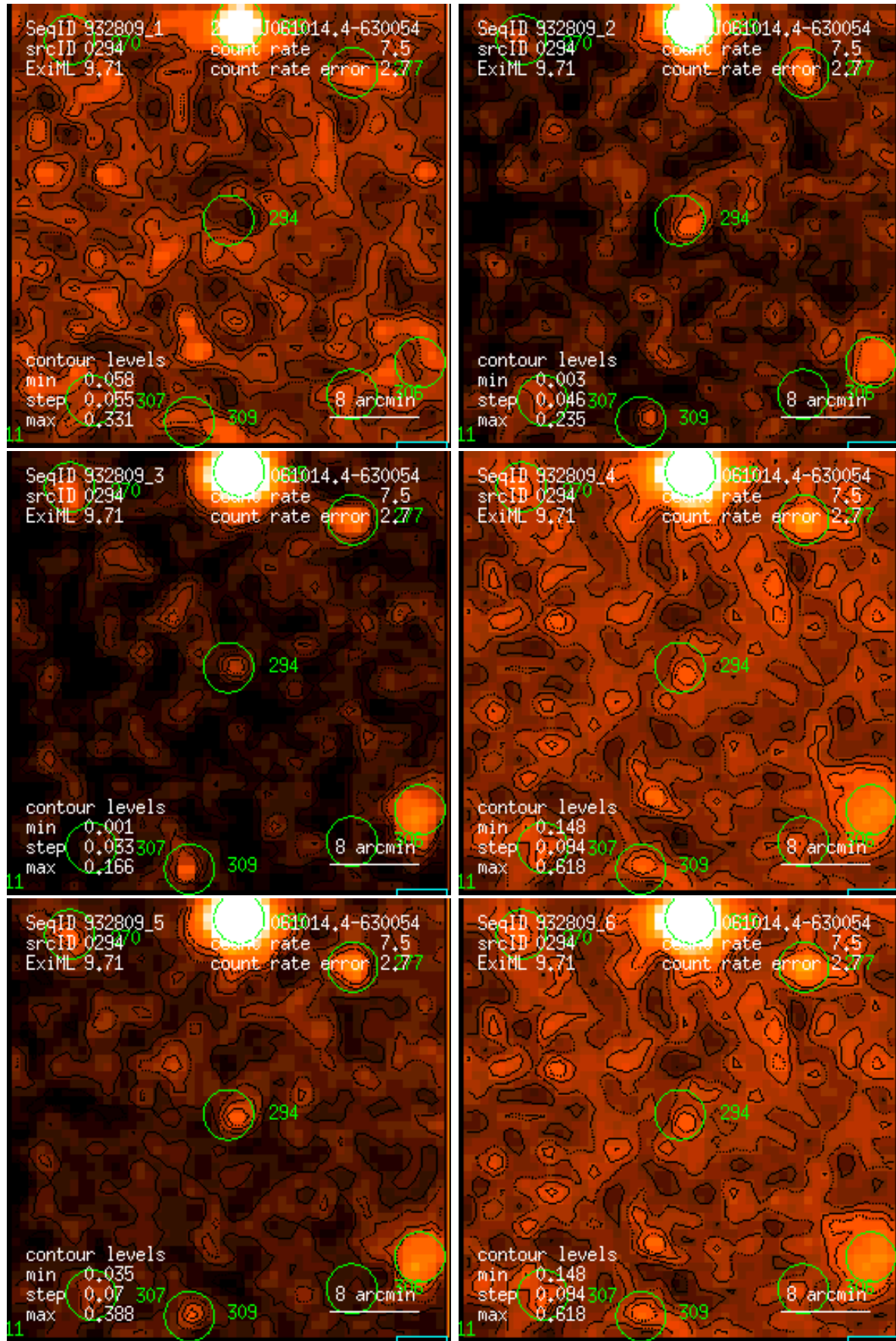
Figure 294: RASS 932809: detection 0294: band rate images, Gaussian filter: (1) PSPC channels 11 – 41, (2) 52 – 90, (3) 91 – 201, (4) 11 – 235, (5) 52 – 201, (6) 11 – 201. Broad band rates in counts/ks. Band rate contour levels in counts/ks/arcmin 2 .
