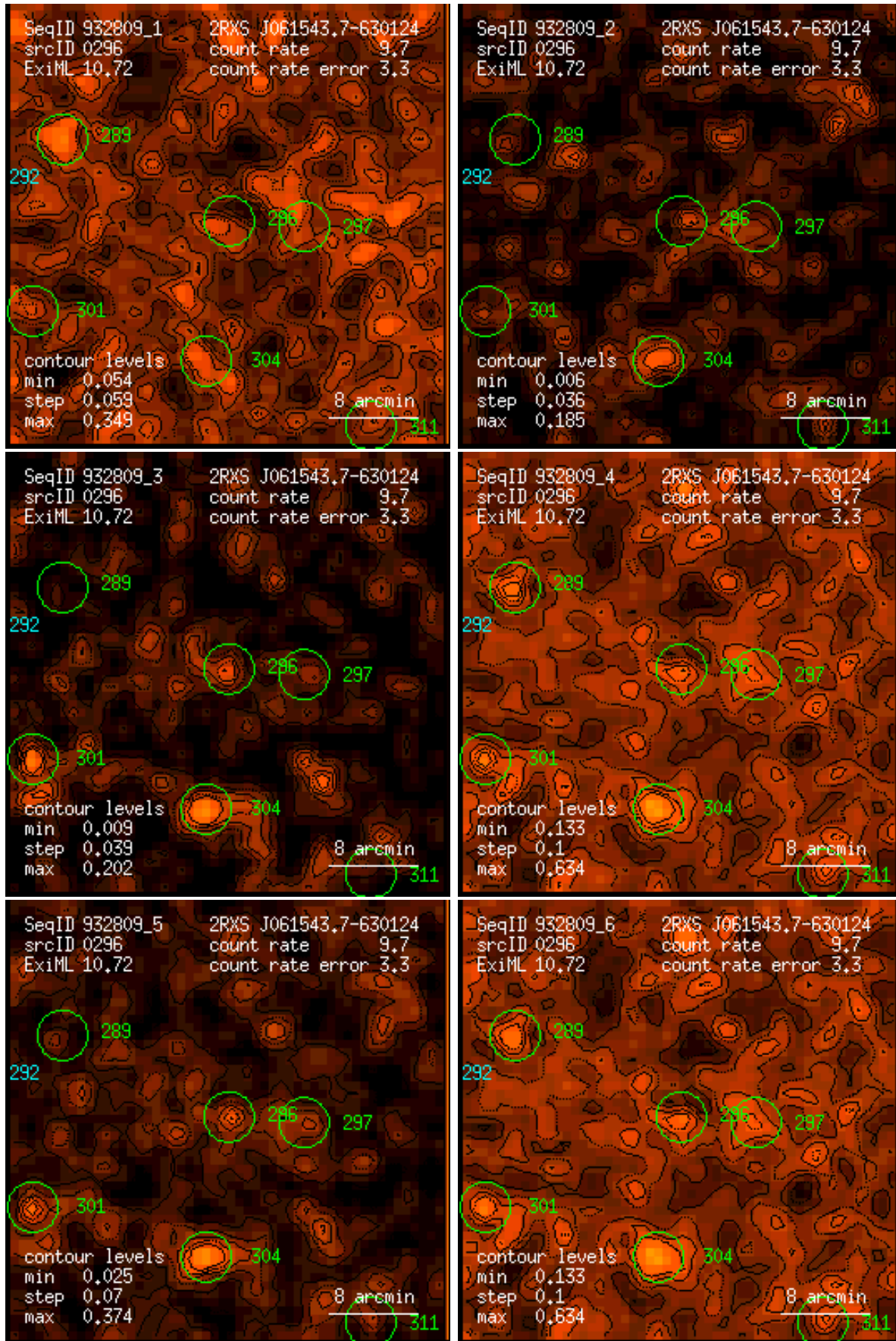
Figure 296: RASS 932809: detection 0296: band rate images, Gaussian filter: (1) PSPC channels 11 – 41, (2) 52 – 90, (3) 91 – 201, (4) 11 – 235, (5) 52 – 201, (6) 11 – 201. Broad band rates in counts/ks. Band rate contour levels in counts/ks/arcmin 2 .
