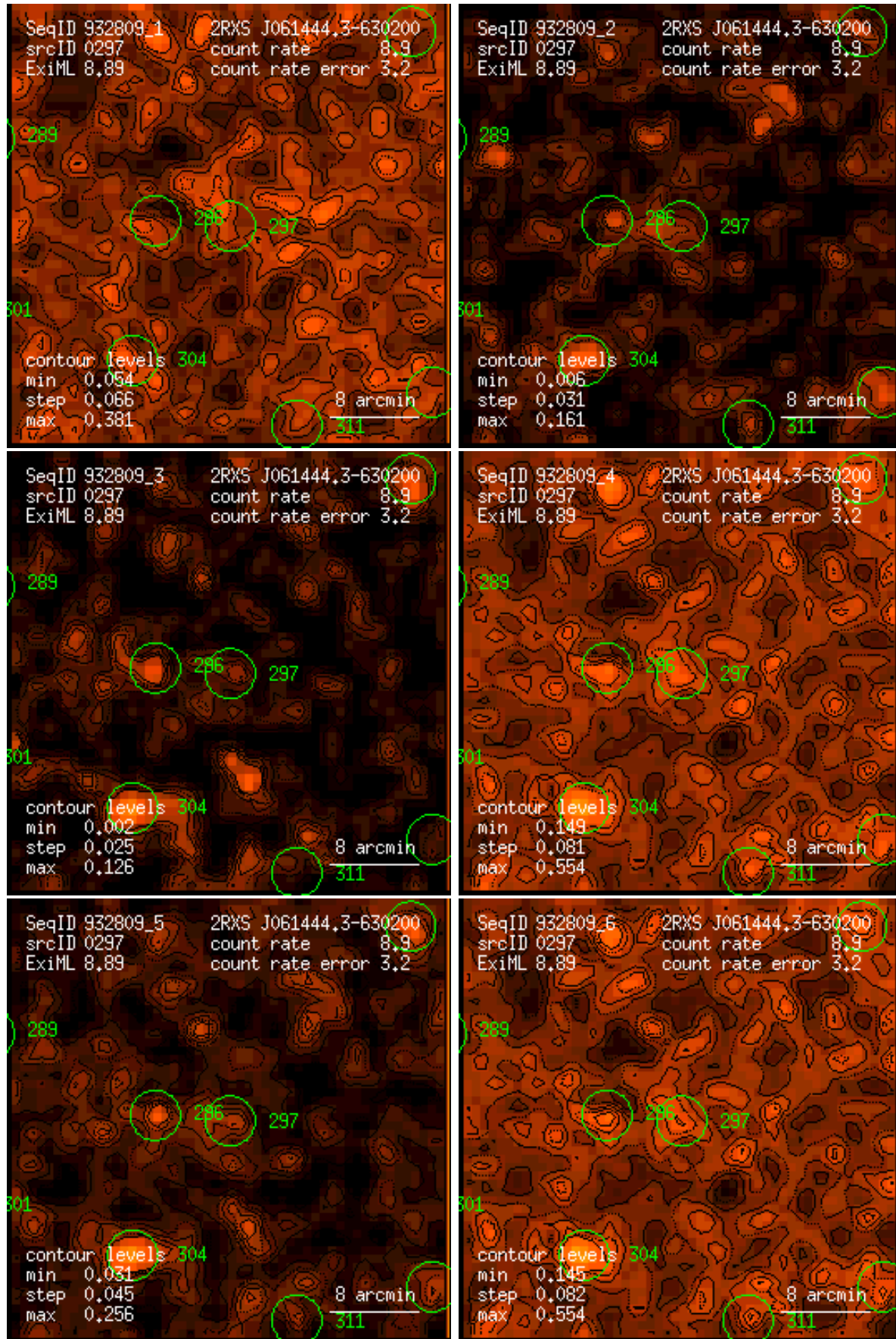
Figure 297: RASS 932809: detection 0297: band rate images, Gaussian filter: (1) PSPC channels 11 – 41, (2) 52 – 90, (3) 91 – 201, (4) 11 – 235, (5) 52 – 201, (6) 11 – 201. Broad band rates in counts/ks. Band rate contour levels in counts/ks/arcmin 2 .
