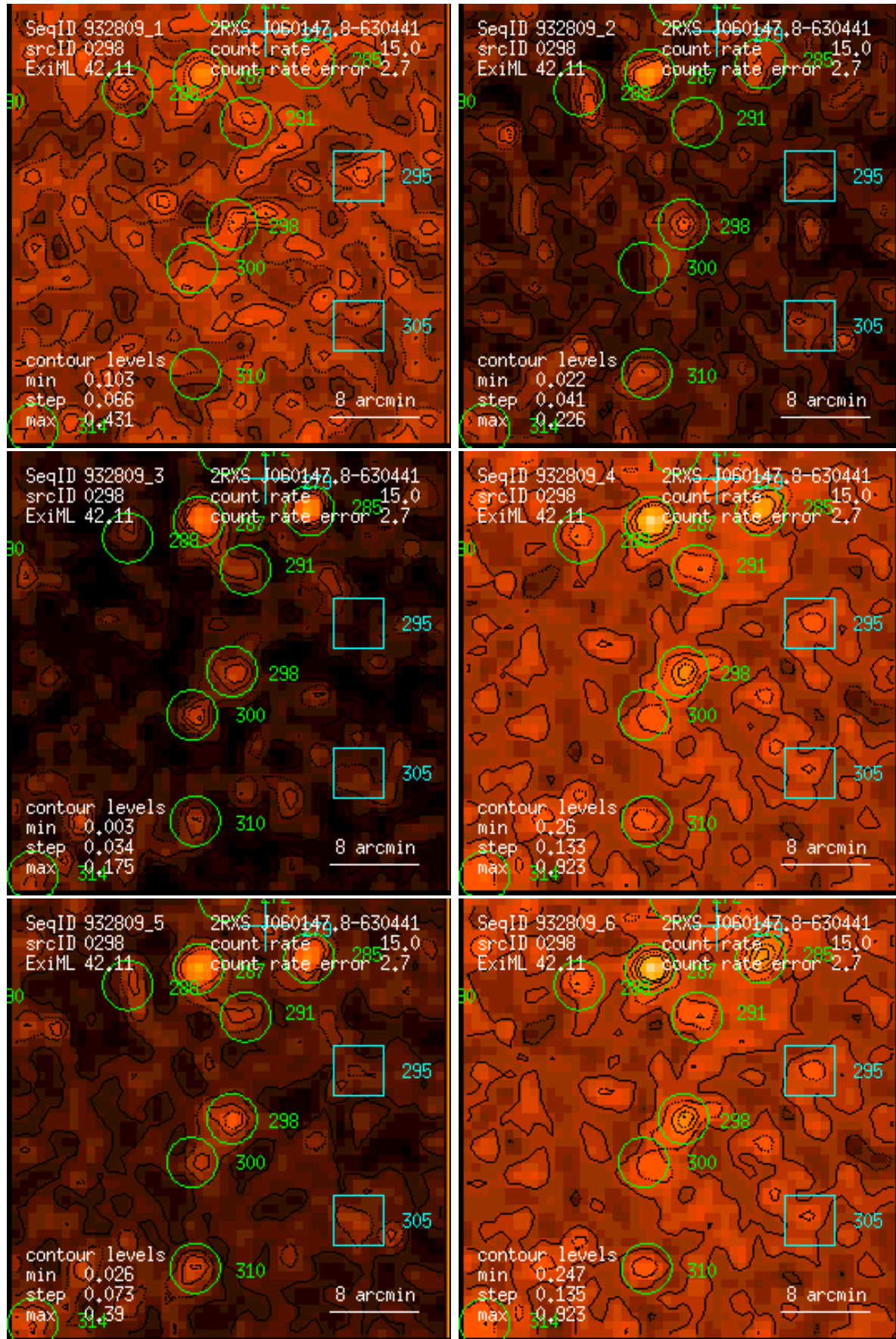
Figure 298: RASS 932809: detection 0298: band rate images, Gaussian filter: (1) PSPC channels 11 – 41, (2) 52 – 90, (3) 91 – 201, (4) 11 – 235, (5) 52 – 201, (6) 11 – 201. Broad band rates in counts/ks. Band rate contour levels in counts/ks/arcmin 2 .
