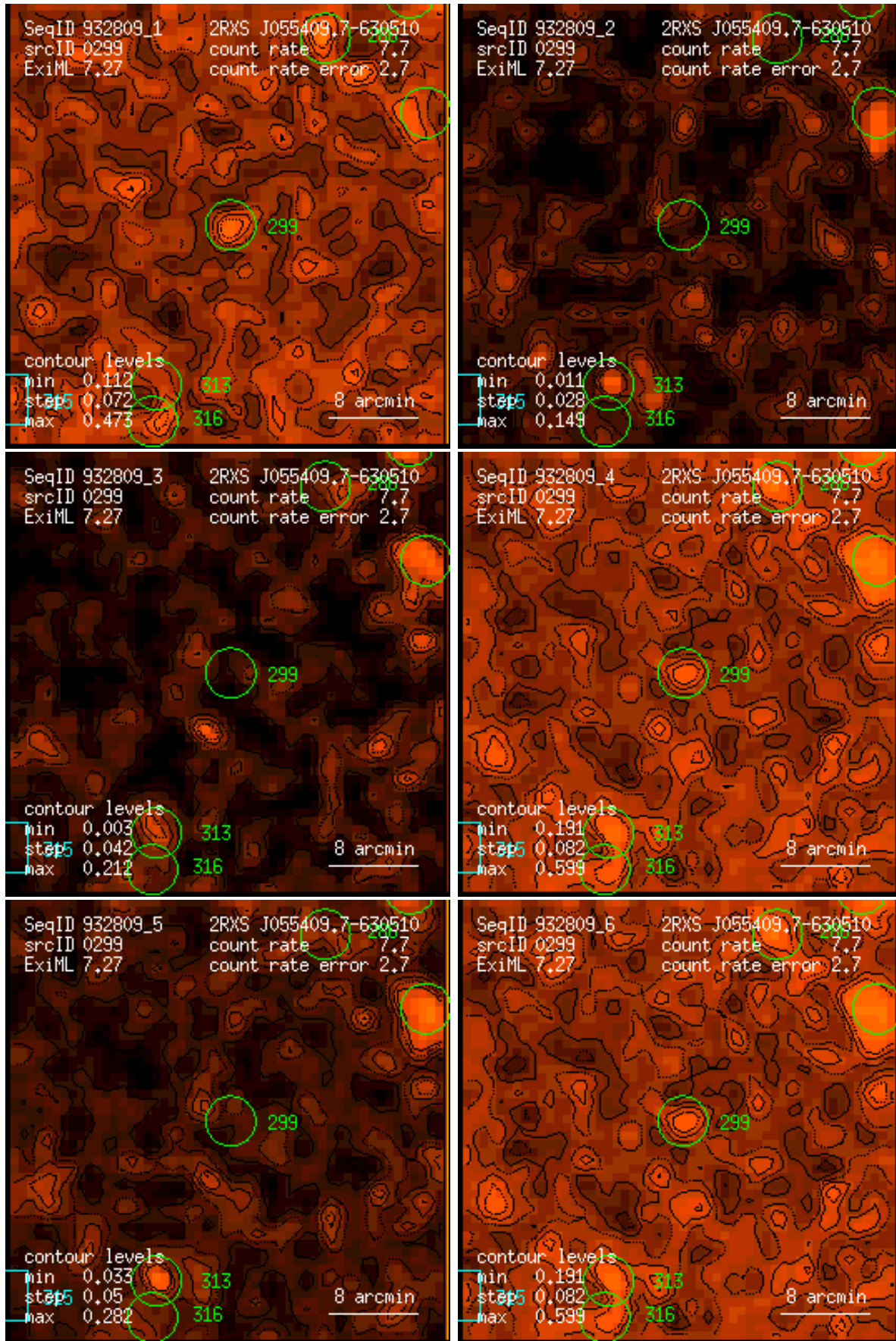
Figure 299: RASS 932809: detection 0299: band rate images, Gaussian filter: (1) PSPC channels 11 – 41, (2) 52 – 90, (3) 91 – 201, (4) 11 – 235, (5) 52 – 201, (6) 11 – 201. Broad band rates in counts/ks. Band rate contour levels in counts/ks/arcmin 2 .
