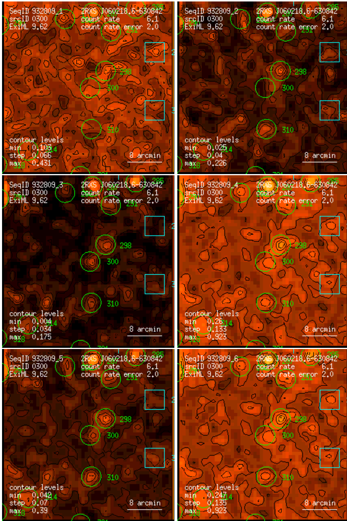
Figure 300: RASS 932809: detection 0300: band rate images, Gaussian filter: (1) PSPC channels 11 – 41, (2) 52 – 90, (3) 91 – 201, (4) 11 – 235, (5) 52 – 201, (6) 11 – 201. Broad band rates in counts/ks. Band rate contour levels in counts/ks/arcmin 2 .
