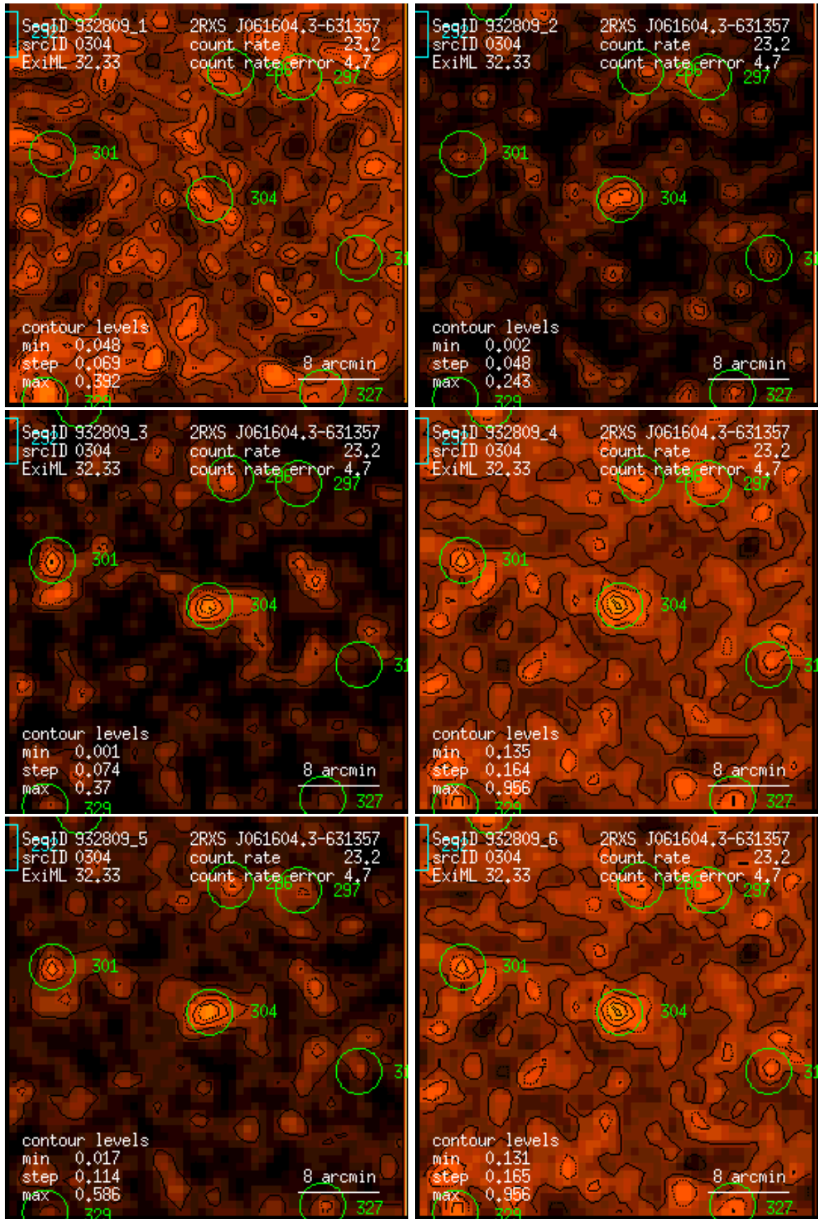
Figure 304: RASS 932809: detection 0304: band rate images, Gaussian filter: (1) PSPC channels 11 – 41, (2) 52 – 90, (3) 91 – 201, (4) 11 – 235, (5) 52 – 201, (6) 11 – 201. Broad band rates in counts/ks. Band rate contour levels in counts/ks/arcmin 2 .
