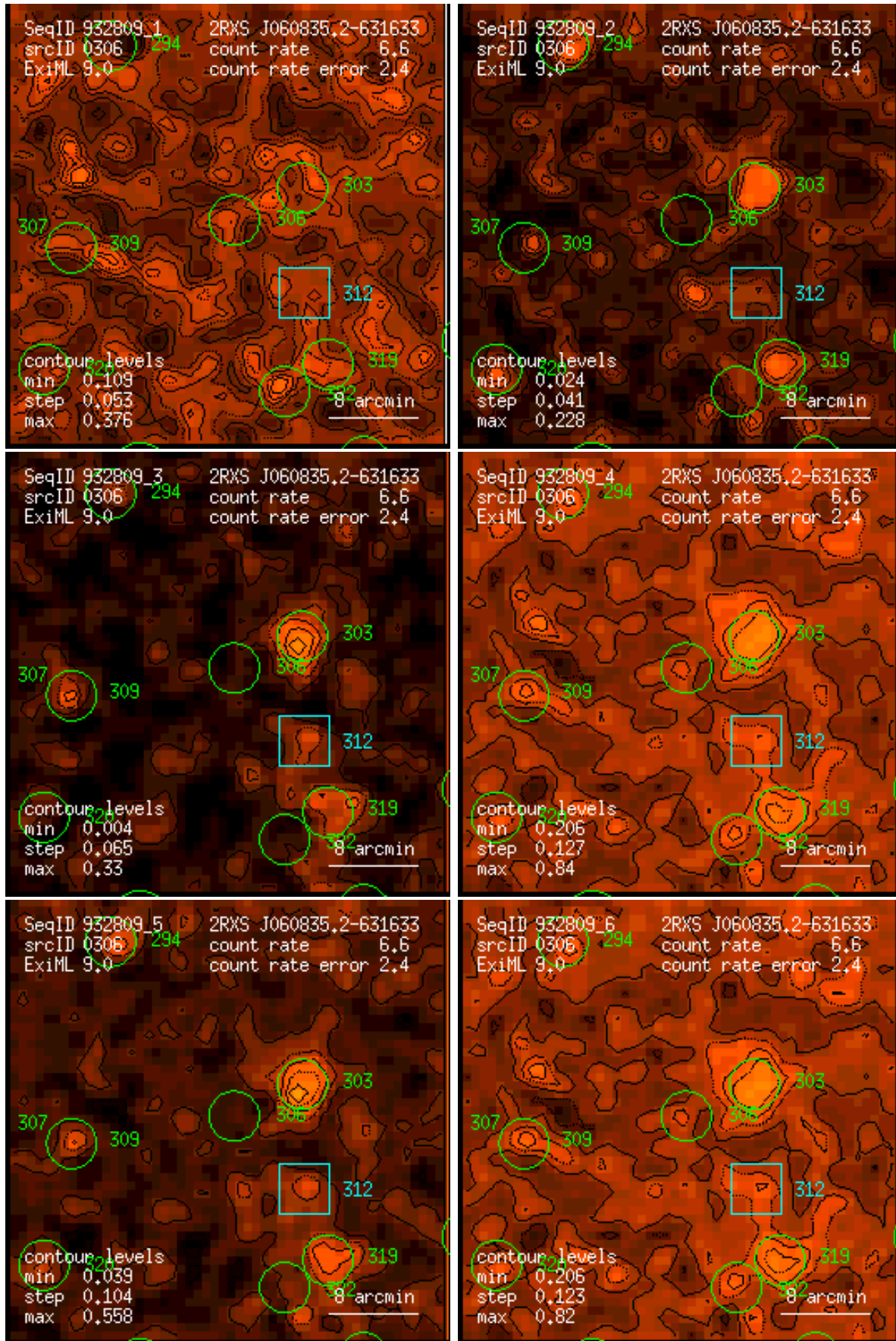
Figure 306: RASS 932809: detection 0306: band rate images, Gaussian filter: (1) PSPC channels 11 – 41, (2) 52 – 90, (3) 91 – 201, (4) 11 – 235, (5) 52 – 201, (6) 11 – 201. Broad band rates in counts/ks. Band rate contour levels in counts/ks/arcmin 2 .
